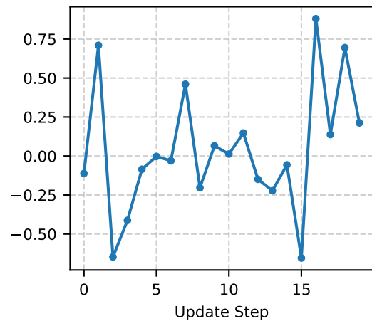
Mean Reward
