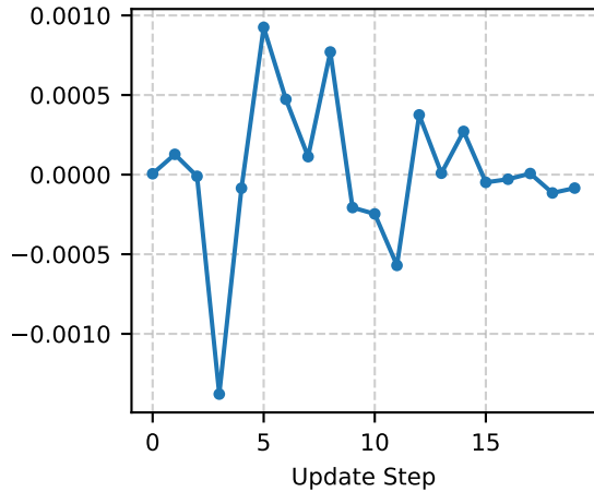
Policy Loss
