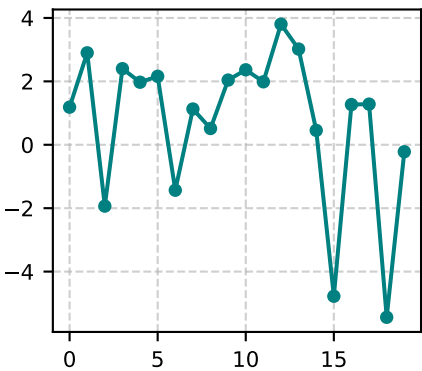
Entropy
