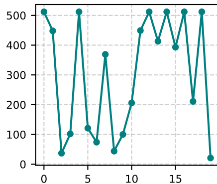
Response Length
