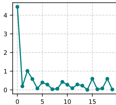
Response Length
