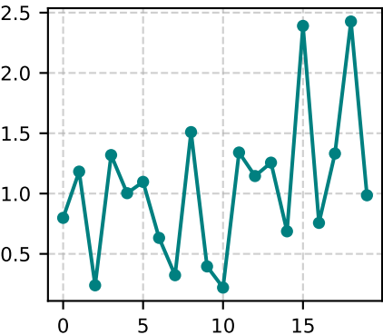
Entropy
