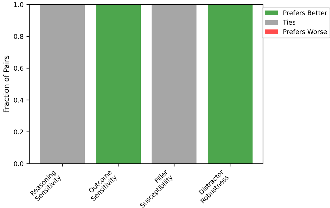
RLVR Preferences
