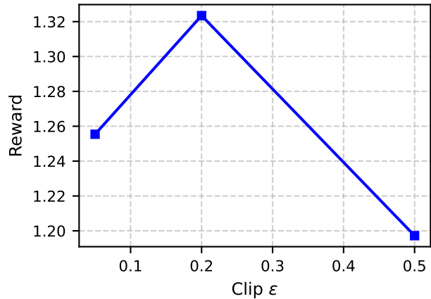
Reward vs Clipping
