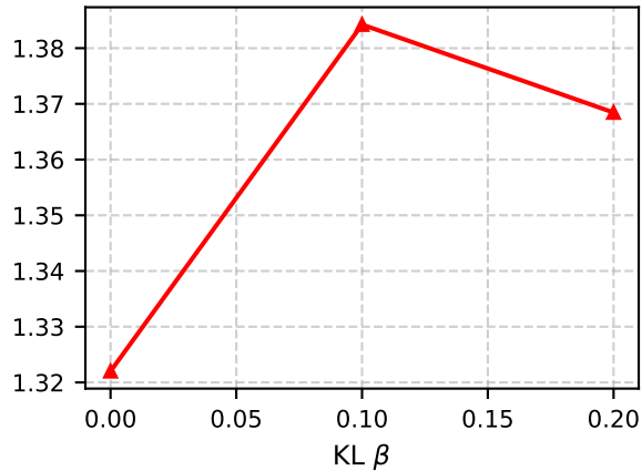
Reward vs KL Penalty
