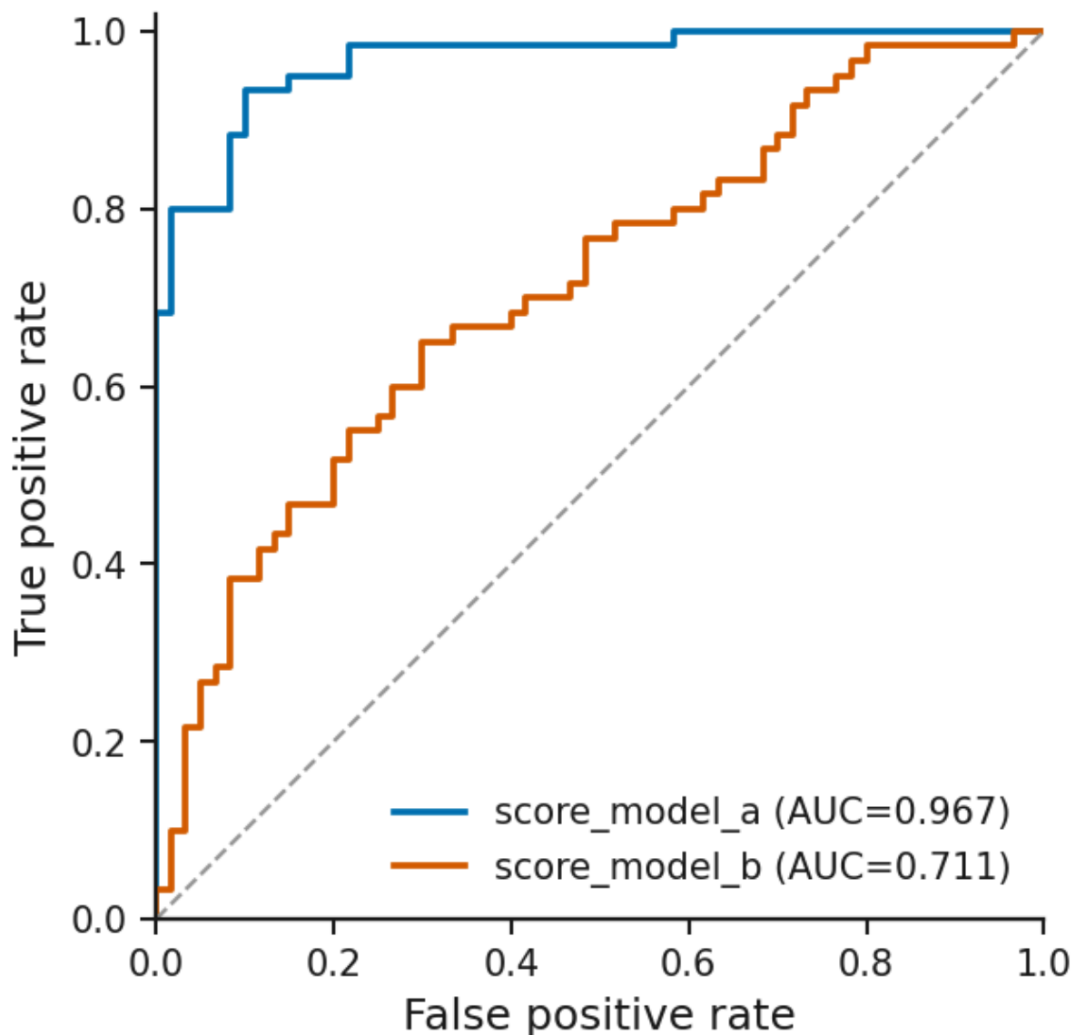
Figure 34. ROC curve: rendered from the bundled synthetic example with Publication defaults.
