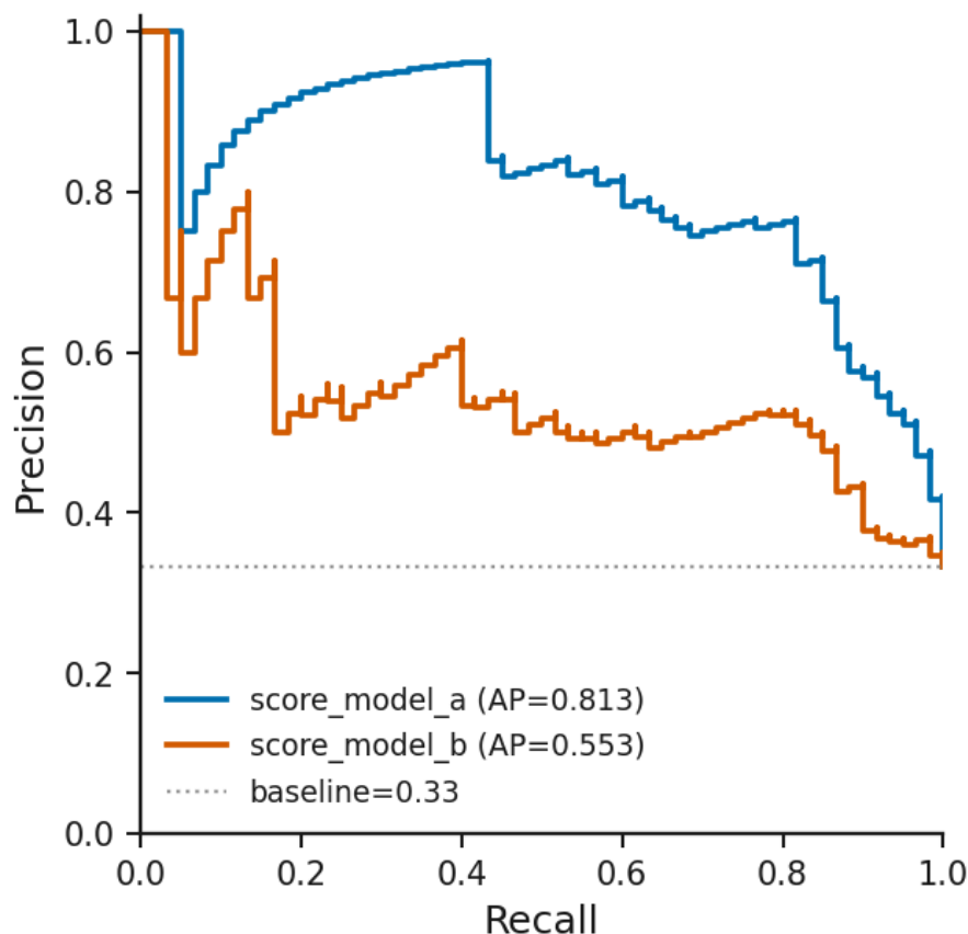
Figure 45. Precision-recall curve: rendered from the bundled synthetic example with Publication defaults.
