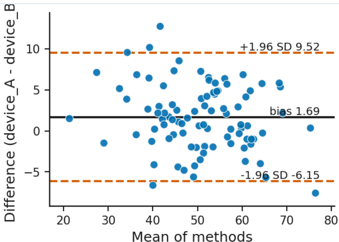
Figure 44. Bland-Altman (method agreement): rendered from the bundled synthetic example with Publication defaults.
