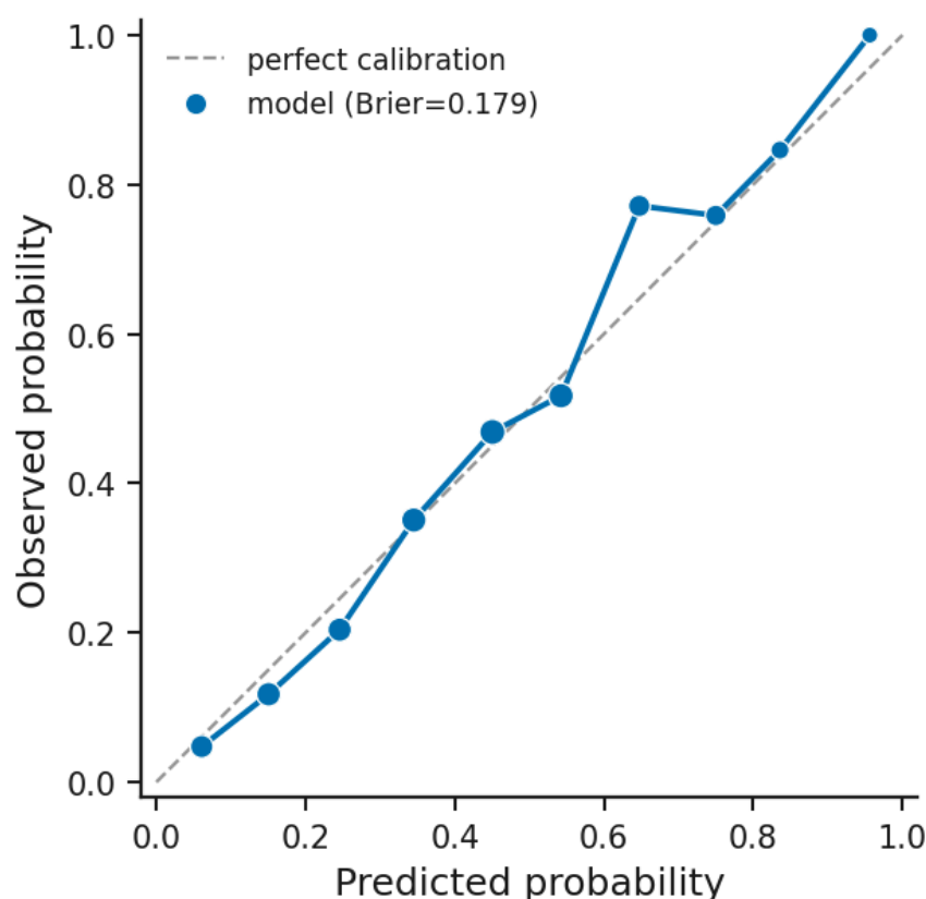
Figure 47. Calibration plot: rendered from the bundled synthetic example with Publication defaults.
