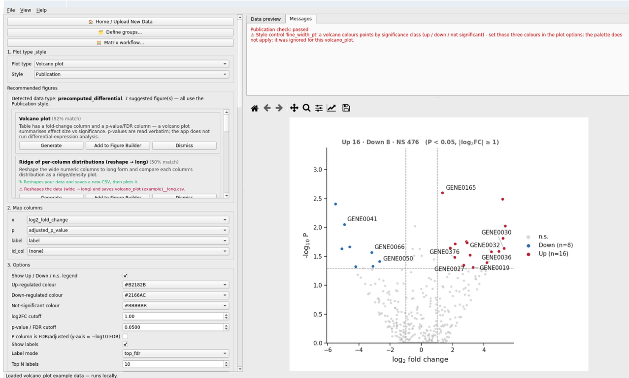
Figure 72. Desktop volcano editor.
