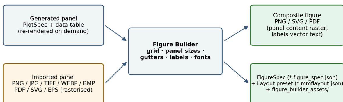
Figure 65. Figure Builder provenance: generated and imported panels, the composite, the FigureSpec and layout preset.
