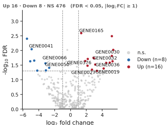
Figure 21. Volcano plot: rendered from the bundled synthetic example with Publication defaults.
