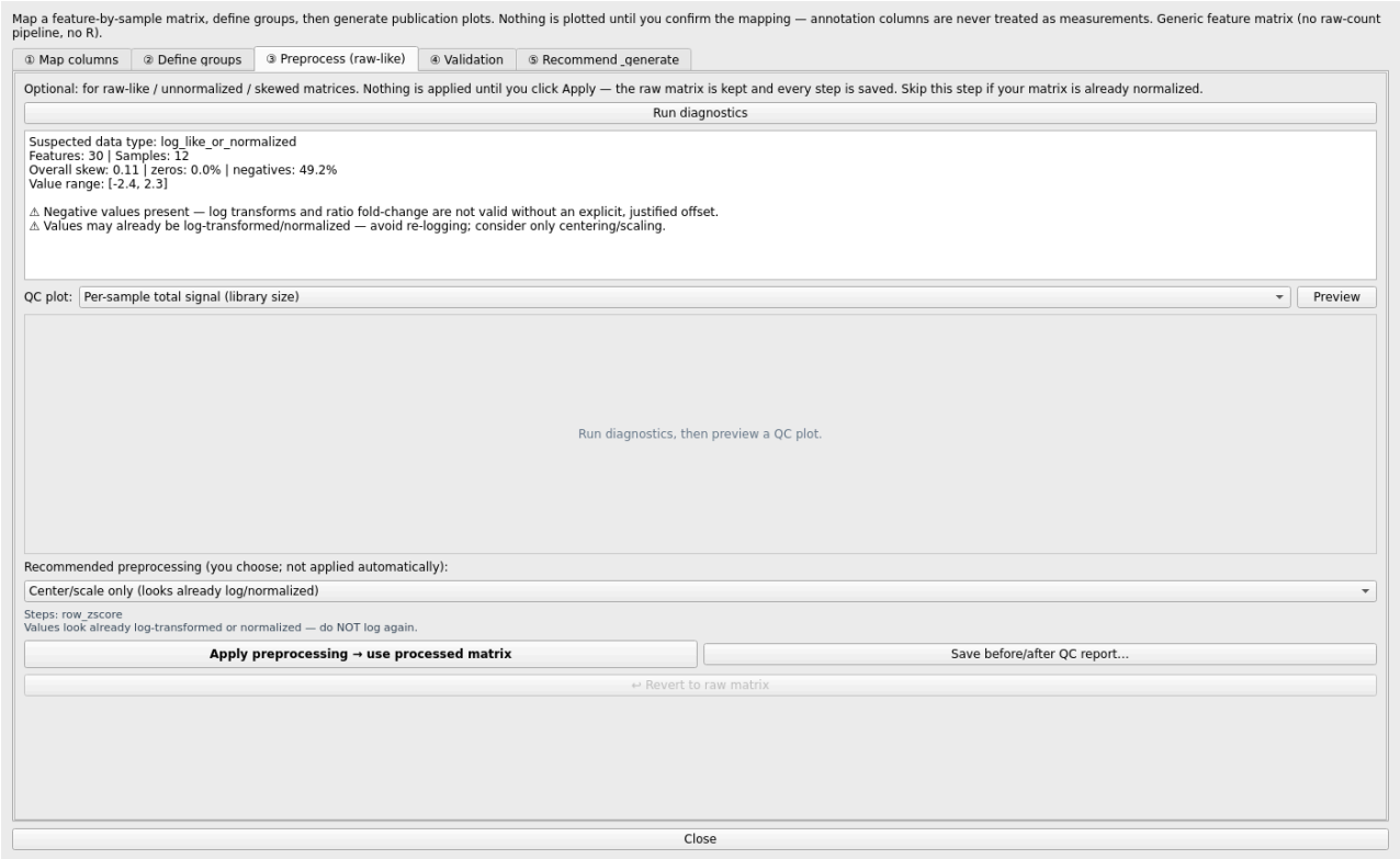
Figure 12. Step ③: Run diagnostics, a QC-plot preview, and the recommended preprocessing recipes (you choose; nothing is applied automatically).
