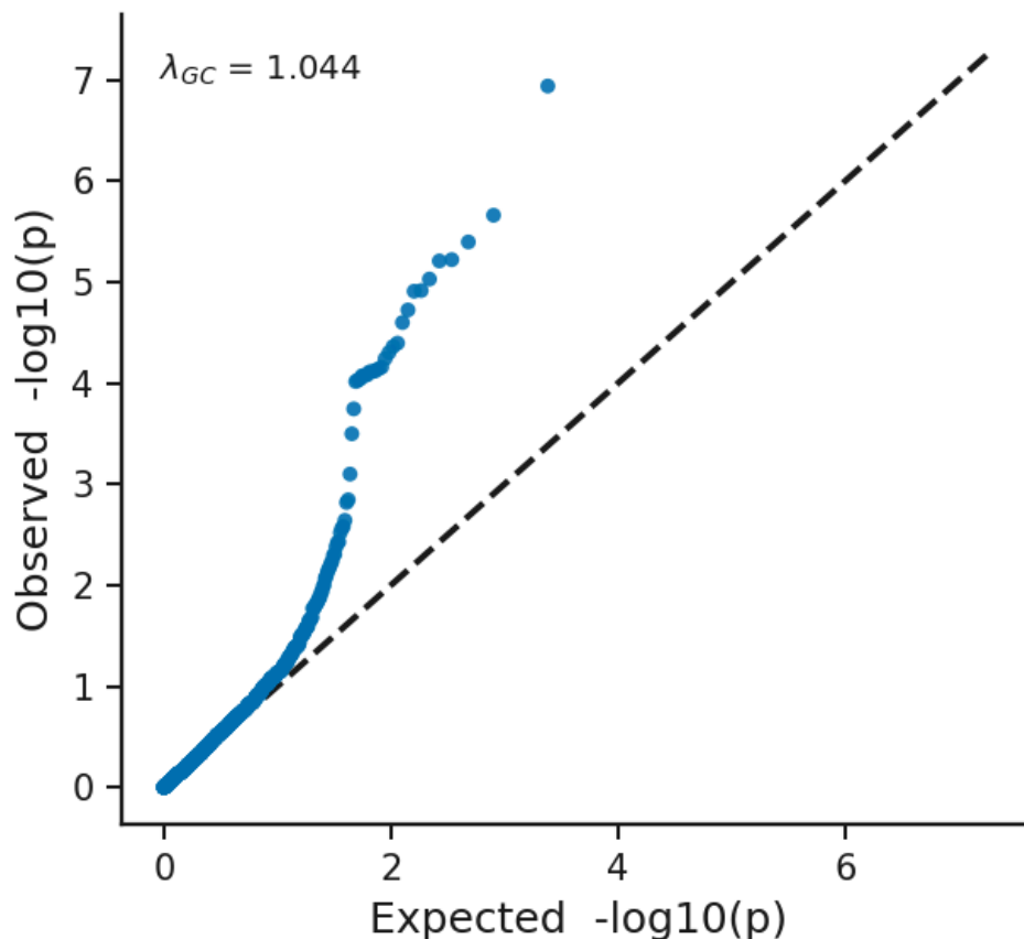
Figure 43. Q-Q plot (p-value / quantile): rendered from the bundled synthetic example with Publication defaults.
