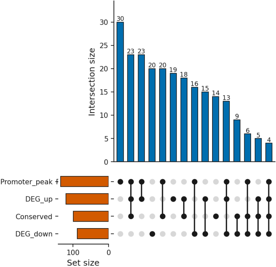
Figure 49. UpSet plot (set intersections): rendered from the bundled synthetic example with Publication defaults.
