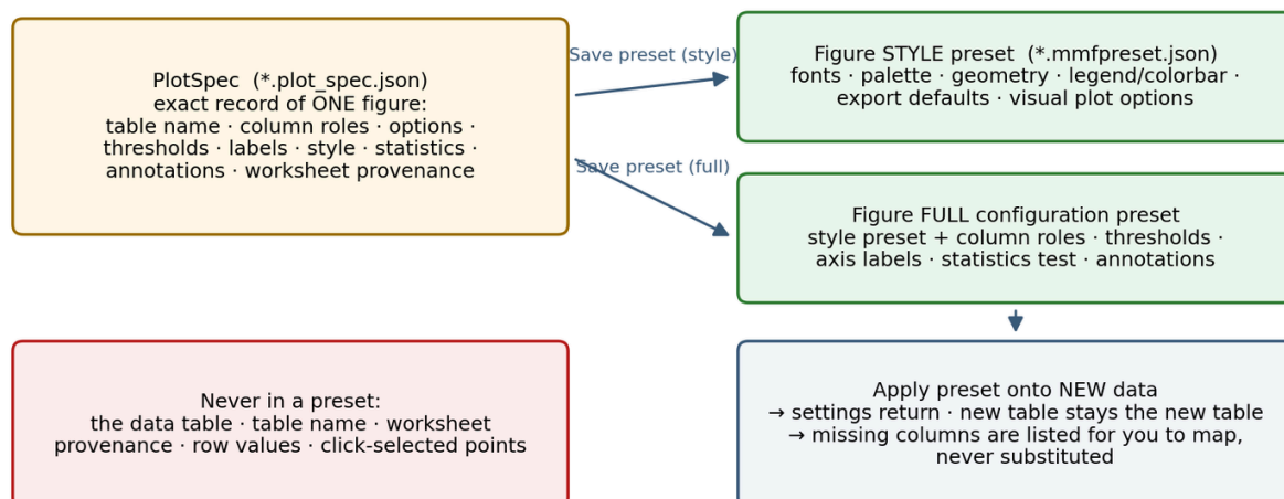
Figure 61. PlotSpec versus Figure preset.
