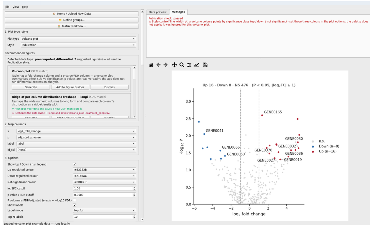
Figure 73. Desktop volcano editor.
