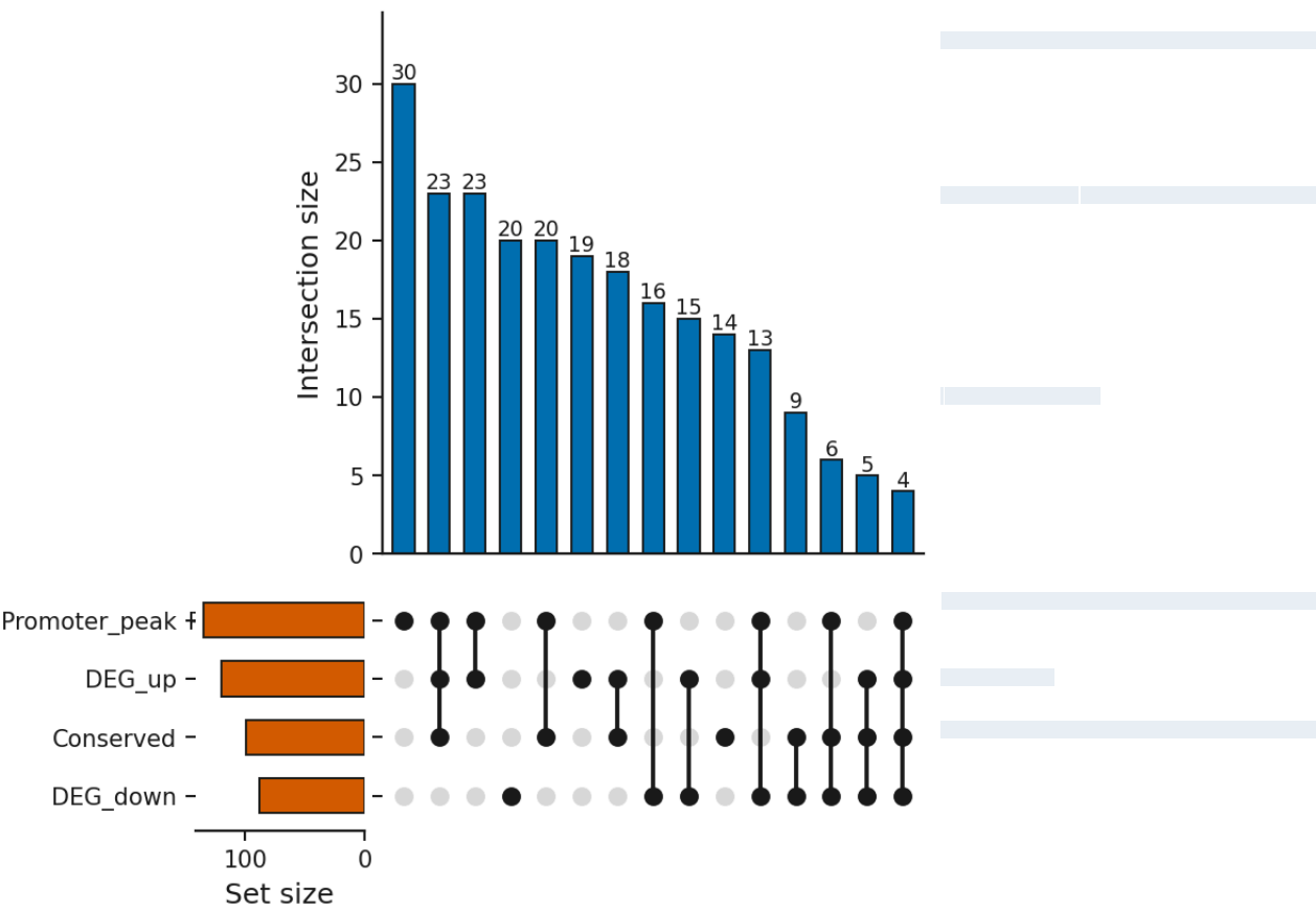
Figure 49. UpSet plot (set intersections): rendered from the bundled synthetic example with Publication defaults.
