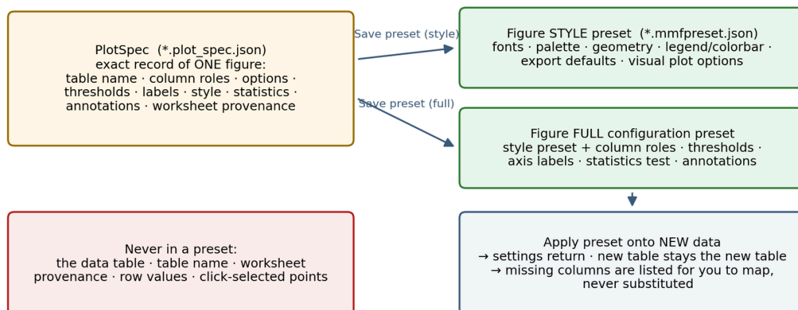
Figure 62. PlotSpec versus Figure preset.
