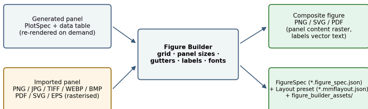
Figure 66. Figure Builder provenance: generated and imported panels, the composite, the FigureSpec and layout preset.
