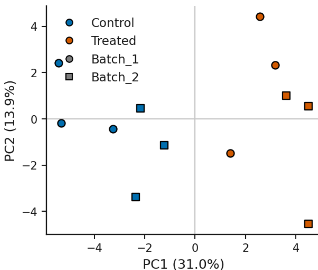
Figure 31. PCA scatter (matrix + metadata): rendered from the bundled synthetic example with Publication defaults.
