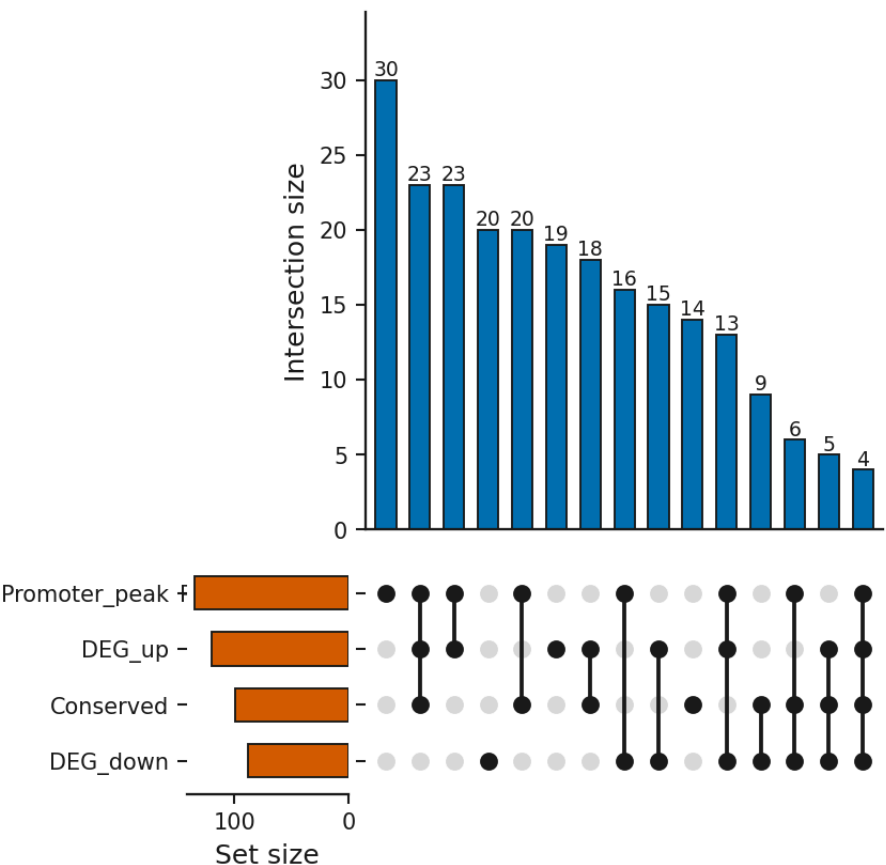
Figure 49. UpSet plot (set intersections): rendered from the bundled synthetic example with Publication defaults.
