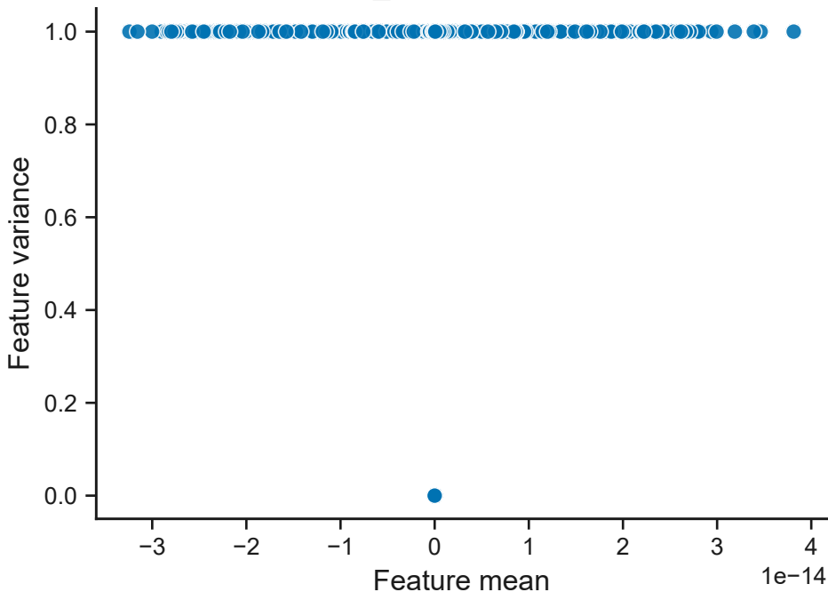
mean_variance — after
