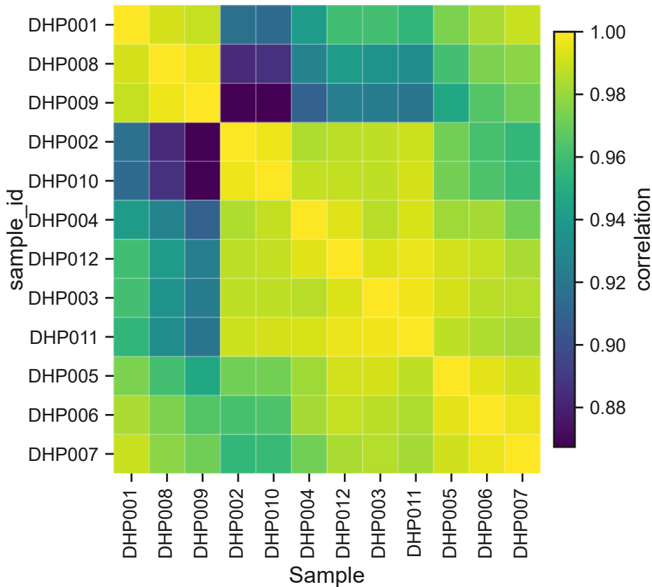
sample_correlation — before
