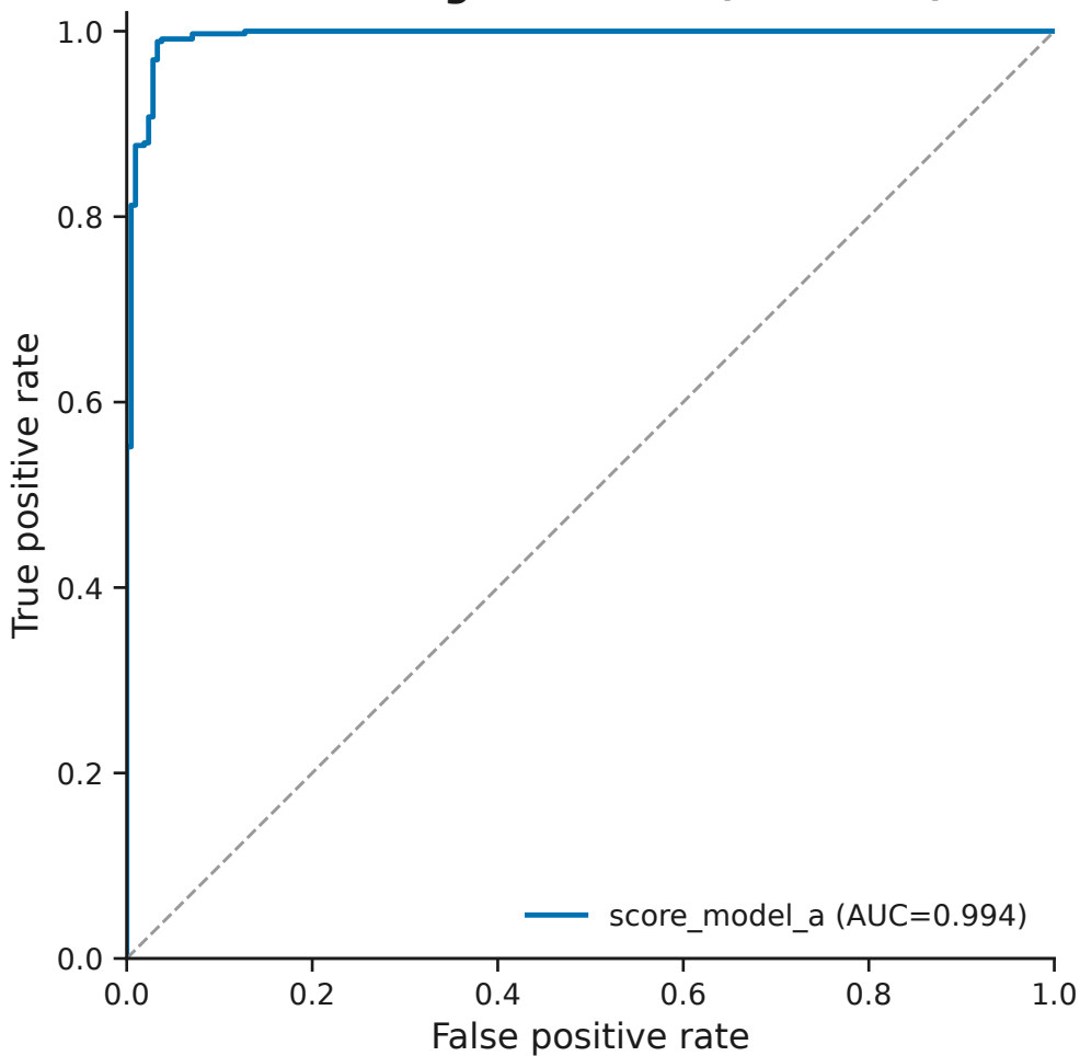
WDBC diagnostic ROC (5-fold CV)
