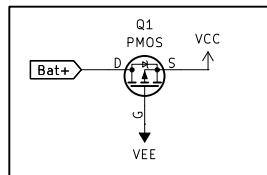
Polarity Protection PMOS
