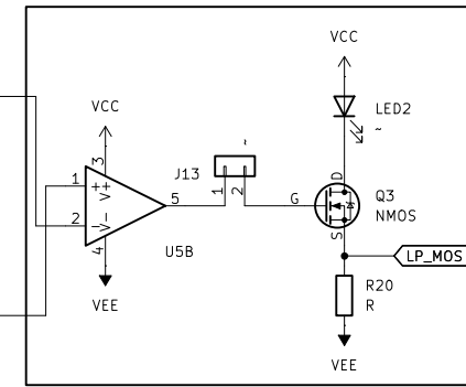
PWM LED Driver
