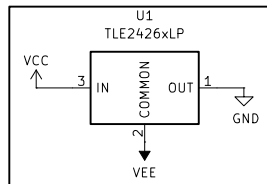
Rail Splitter
