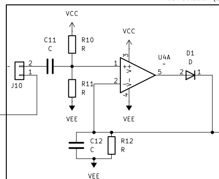
Peak Detector (HP)
