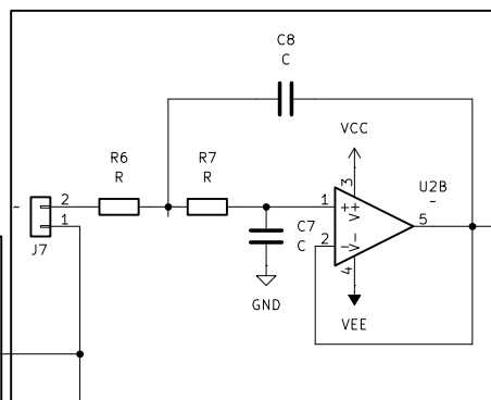
Sallen-Key Low-Pass Filter
