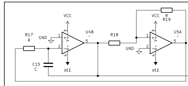
Triangle-Wave Oscillator
