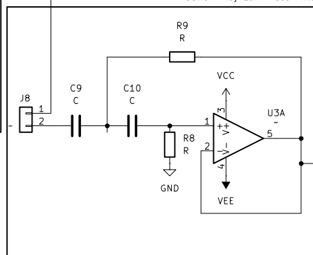
Sallen-Key High-Pass Filter
