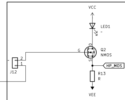
Analog LED Driver
