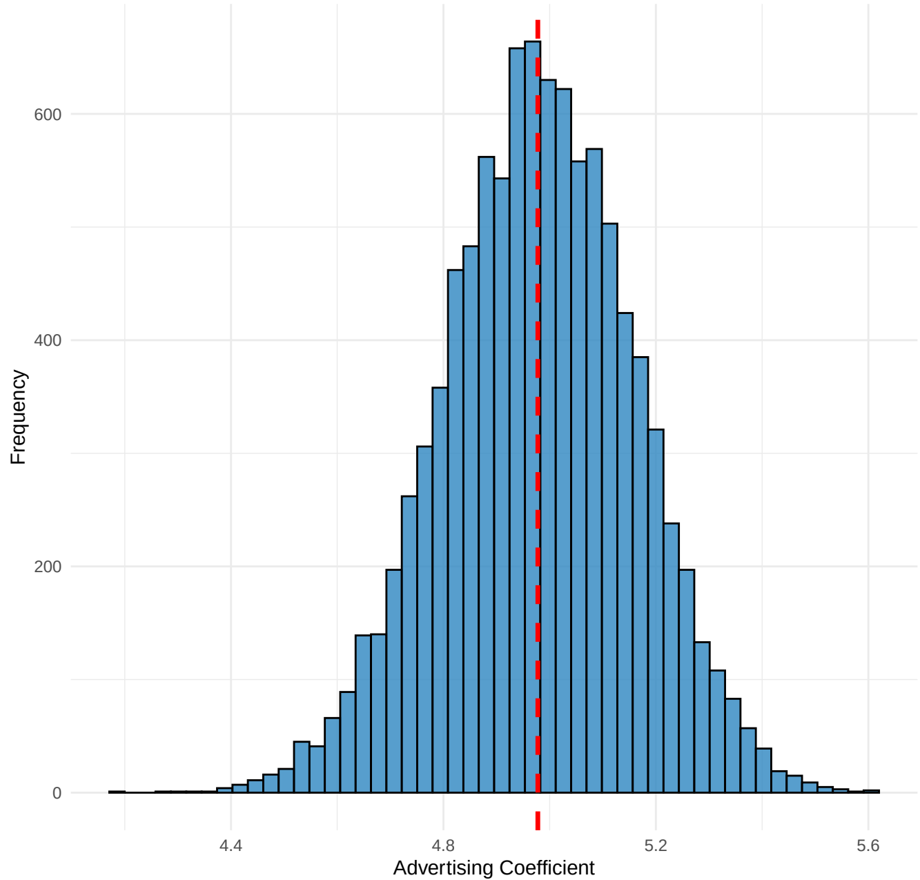
Bootstrap Distribution: Effect of Advertising on Sales
