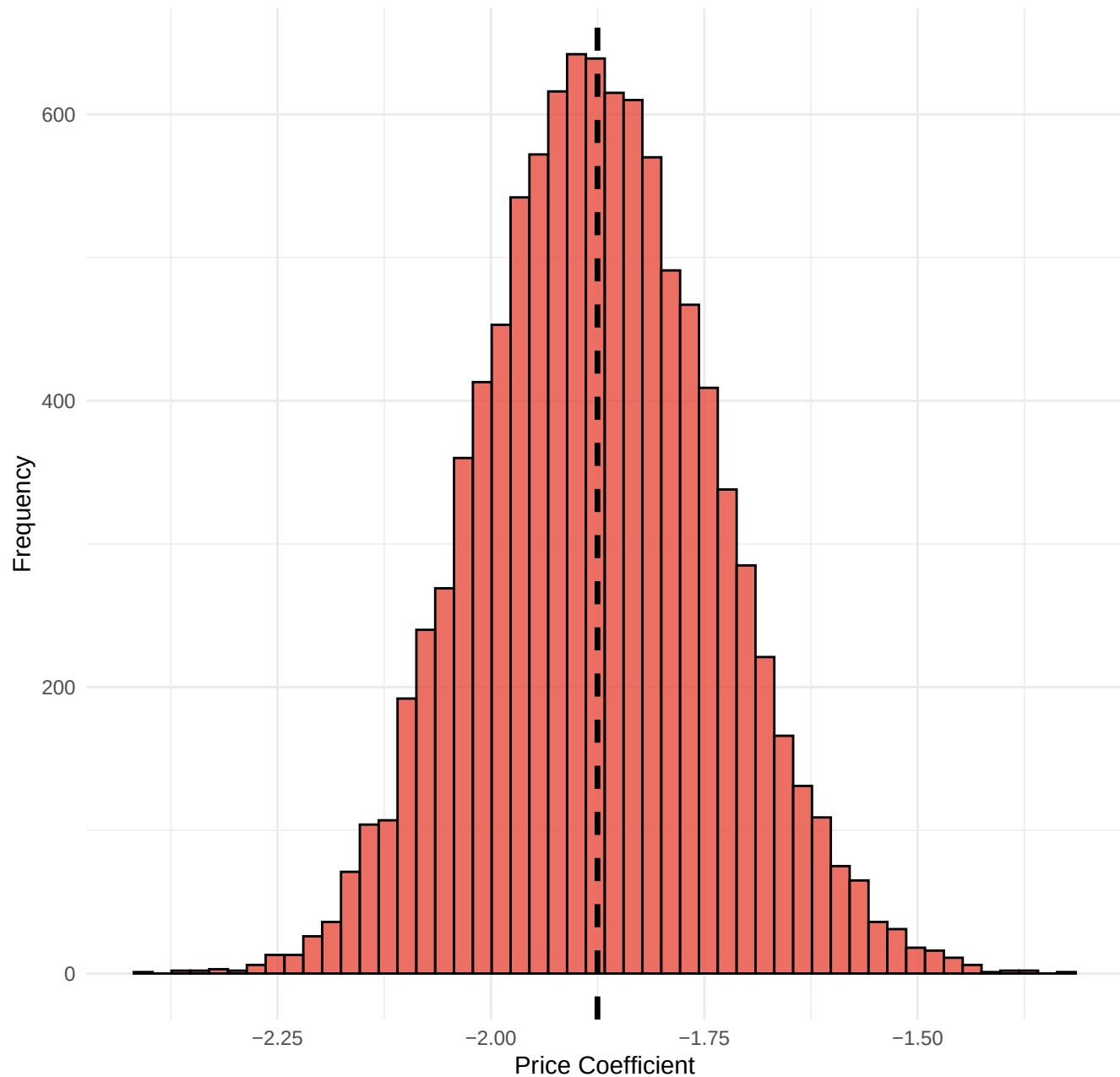
Bootstrap Distribution: Effect of Price on Sales
