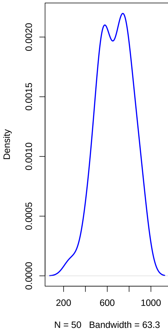
Density Plot of Sales
