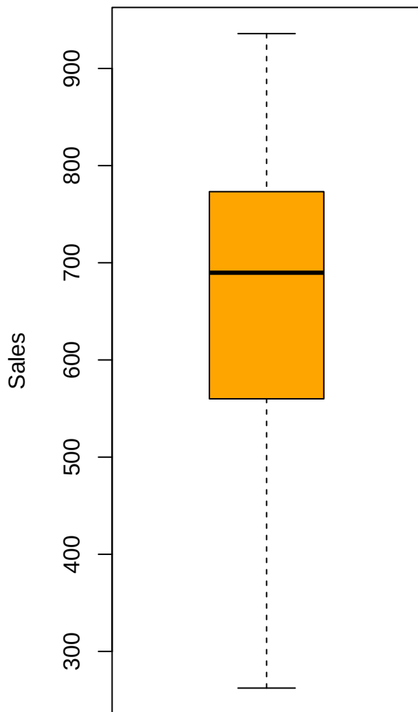
Boxplot of Sales
