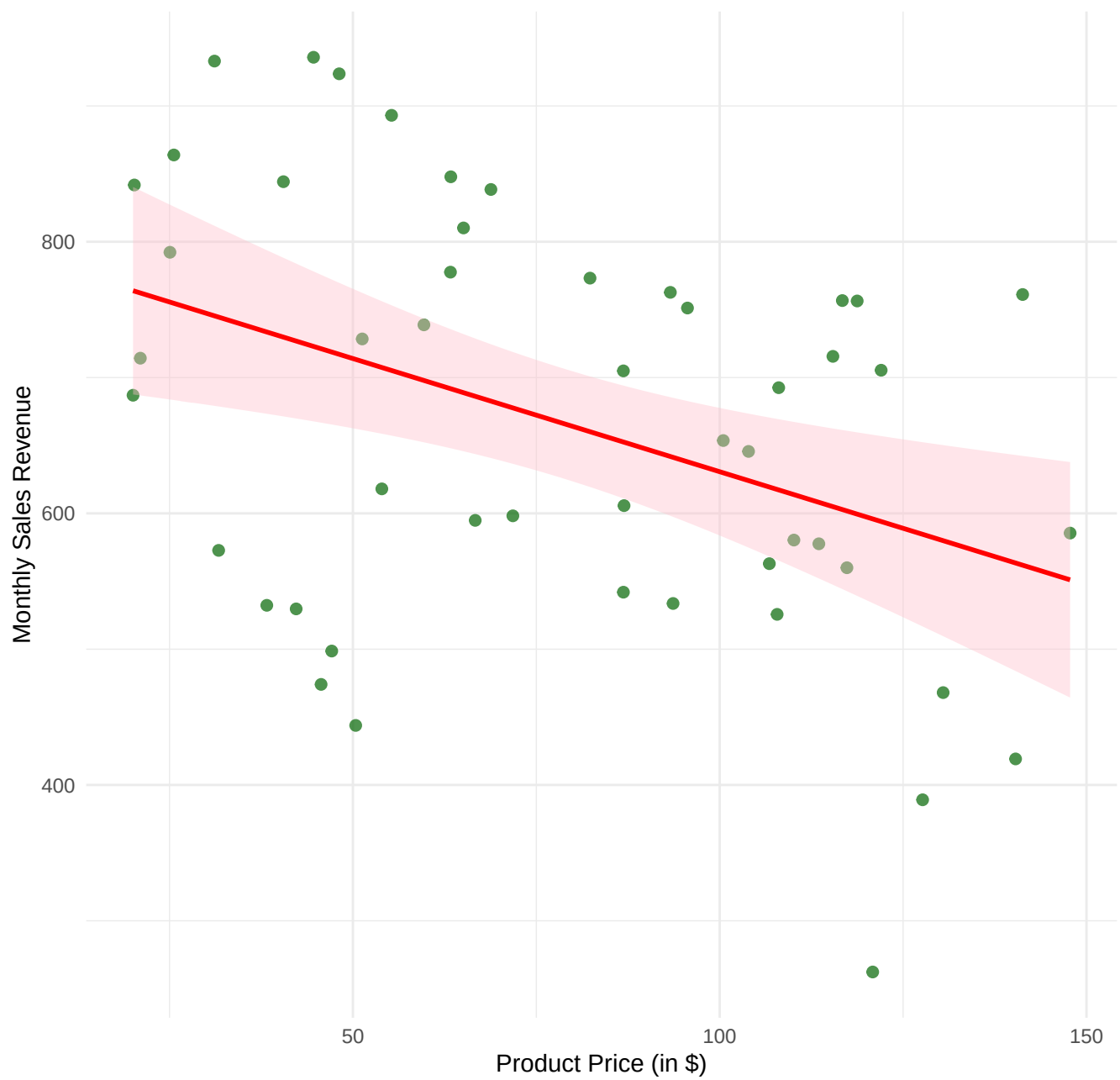
Fitted Linear Model: Sales vs Product Price
