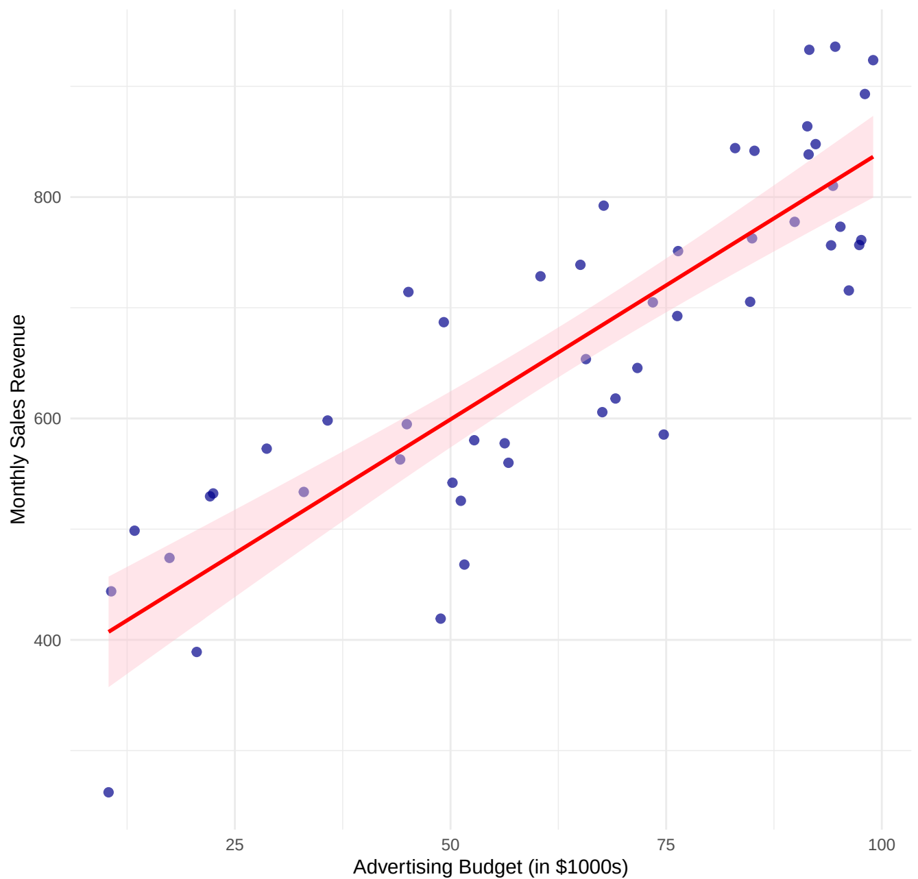
Fitted Linear Model: Sales vs Advertising
