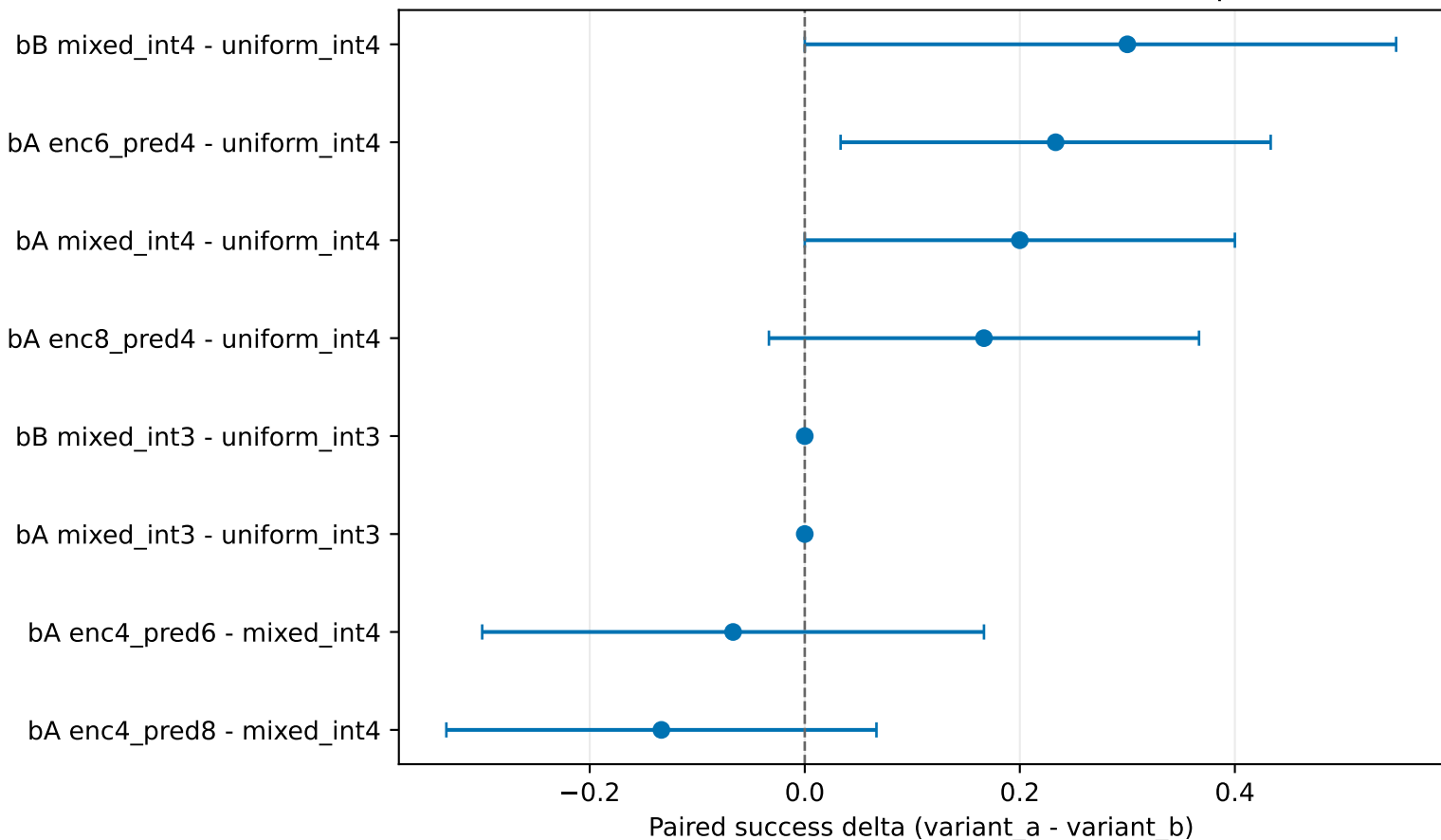
Paired mixed-bit effects with 95% bootstrap CI
