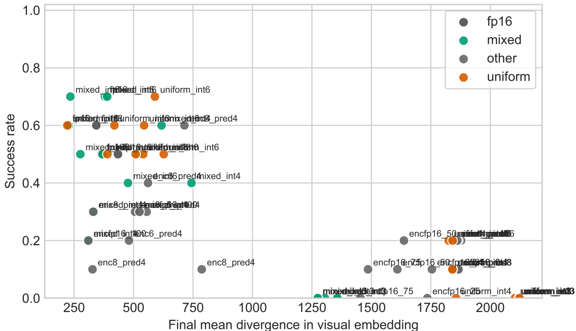
Mechanistic signal: embedding divergence vs planning success
