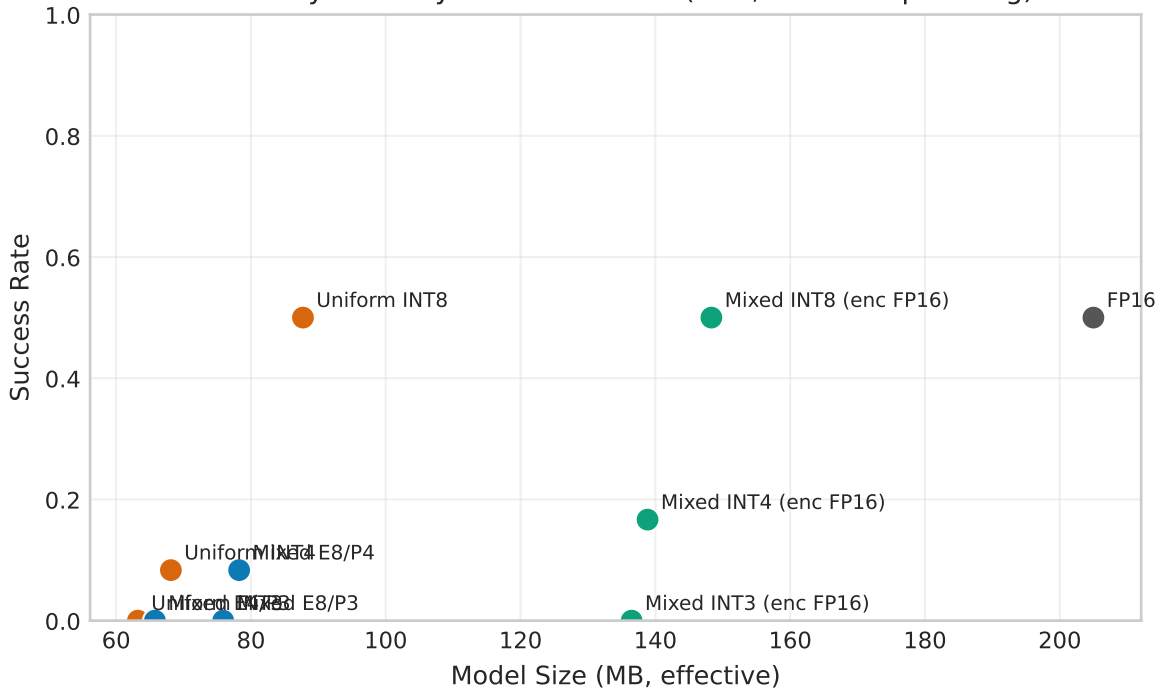
Accuracy-memory frontier on Wall (Mac, bounded planning)
