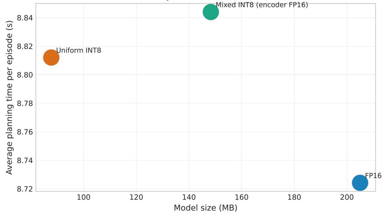
Efficiency tradeoff (Wall, Mac MPS)
