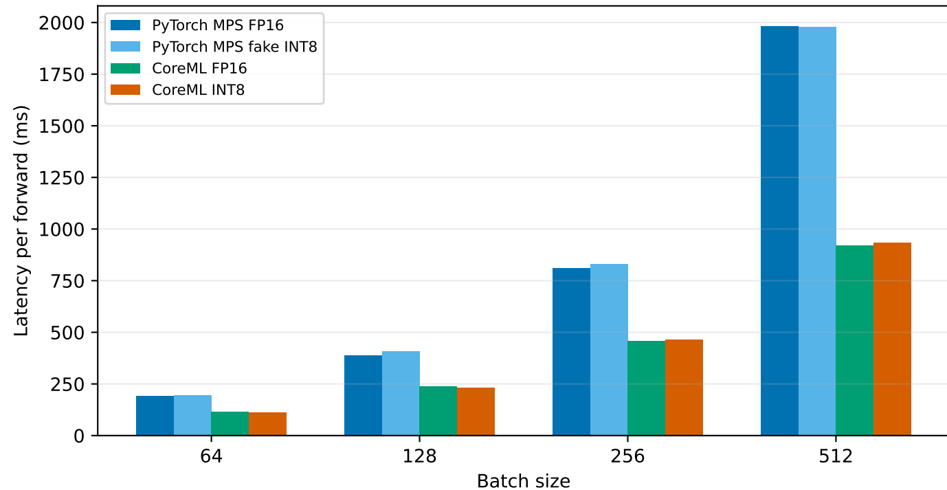
DINO-WM predictor latency on M4 MacBook Pro
