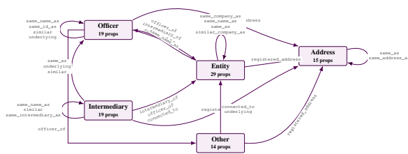
Figure 9: ICIJ Offshore Leaks schema graph used for the third-graph onboarding audit. The schema is compact in node labels but large in edge volume: relationship families encode officer/entity/intermediary roles, registered addresses, identity-resolution links, and similarity links.
