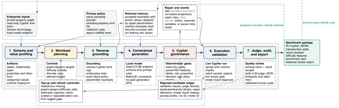
Figure 1: PIPE-Cypher benchmark generation pipeline. The key industry additions beyond static Text2Cypher dataset construction are privacy/value policies, reverse grounding, Cypher governance, execution diagnostics, local judge calibration, and benchmark export/refresh.
