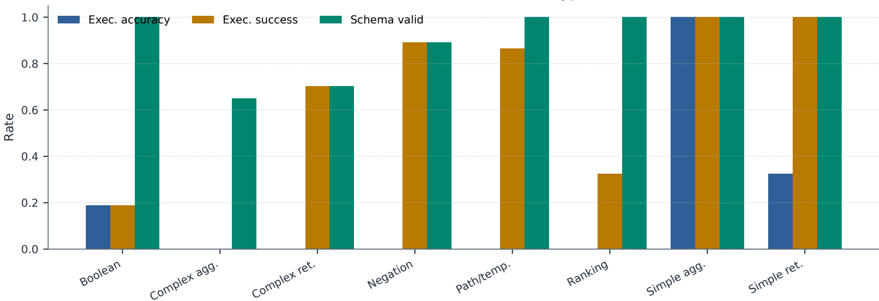
Downstream Qwen3.5-9B zero-shot Text2Cypher breakdown
