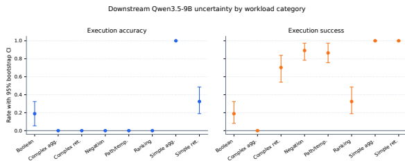
Figure 6: Bootstrap uncertainty for downstream Qwen3.5-9B Text2Cypher evaluation by workload category. Error bars show 95% row-level bootstrap intervals over the full exported test split.
