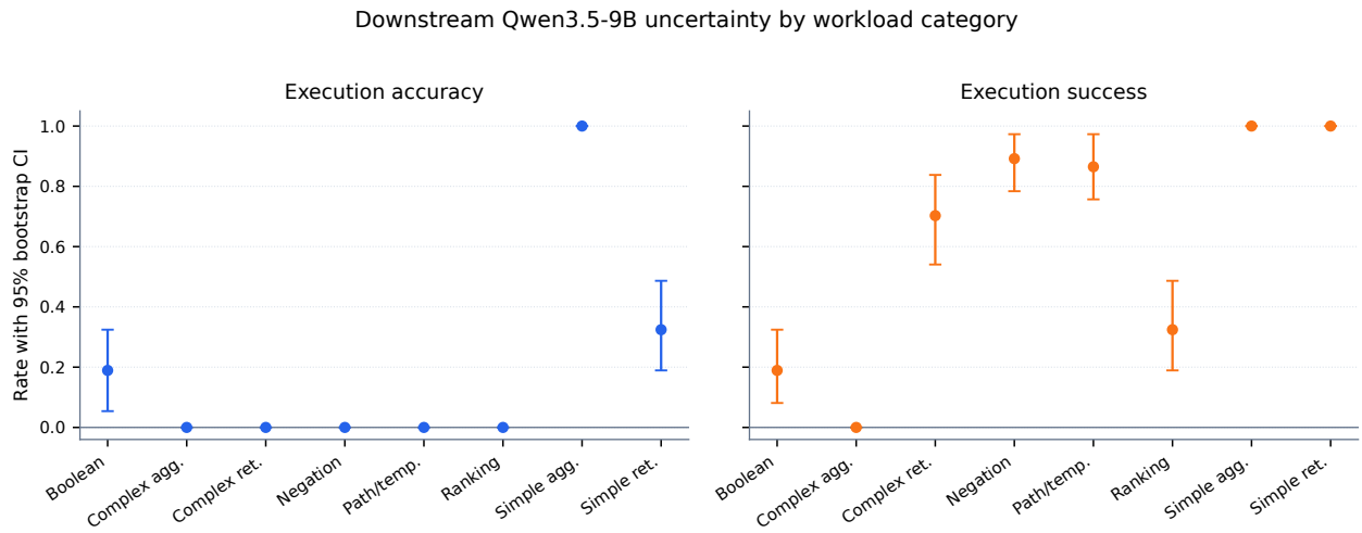
Figure 8: Bootstrap uncertainty for downstream Qwen3.5-9B Text2Cypher evaluation by workload category. Error bars show 95% row-level bootstrap intervals over the full exported test split.
