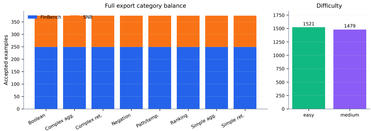
Figure 7: Full 3,000-example export distribution. The benchmark preserves the planned 2:1 FinBench/SNB graph mix while balancing all eight Cypher workload categories and maintaining a near-even easy/medium difficulty split.
