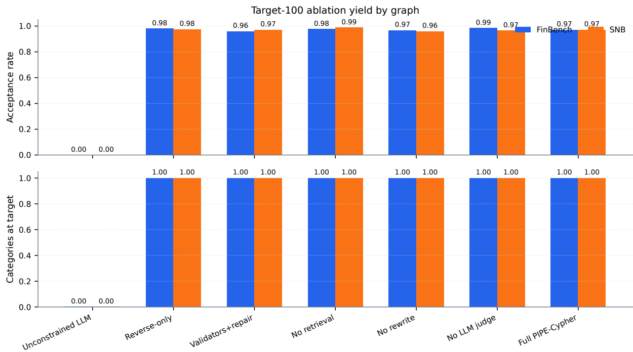
Figure 3: Audited target-100 ablation suite over FinBench and SNB. Every non-unconstrained graph/setting cell reaches all eight category targets with 800 accepted examples per cell.
