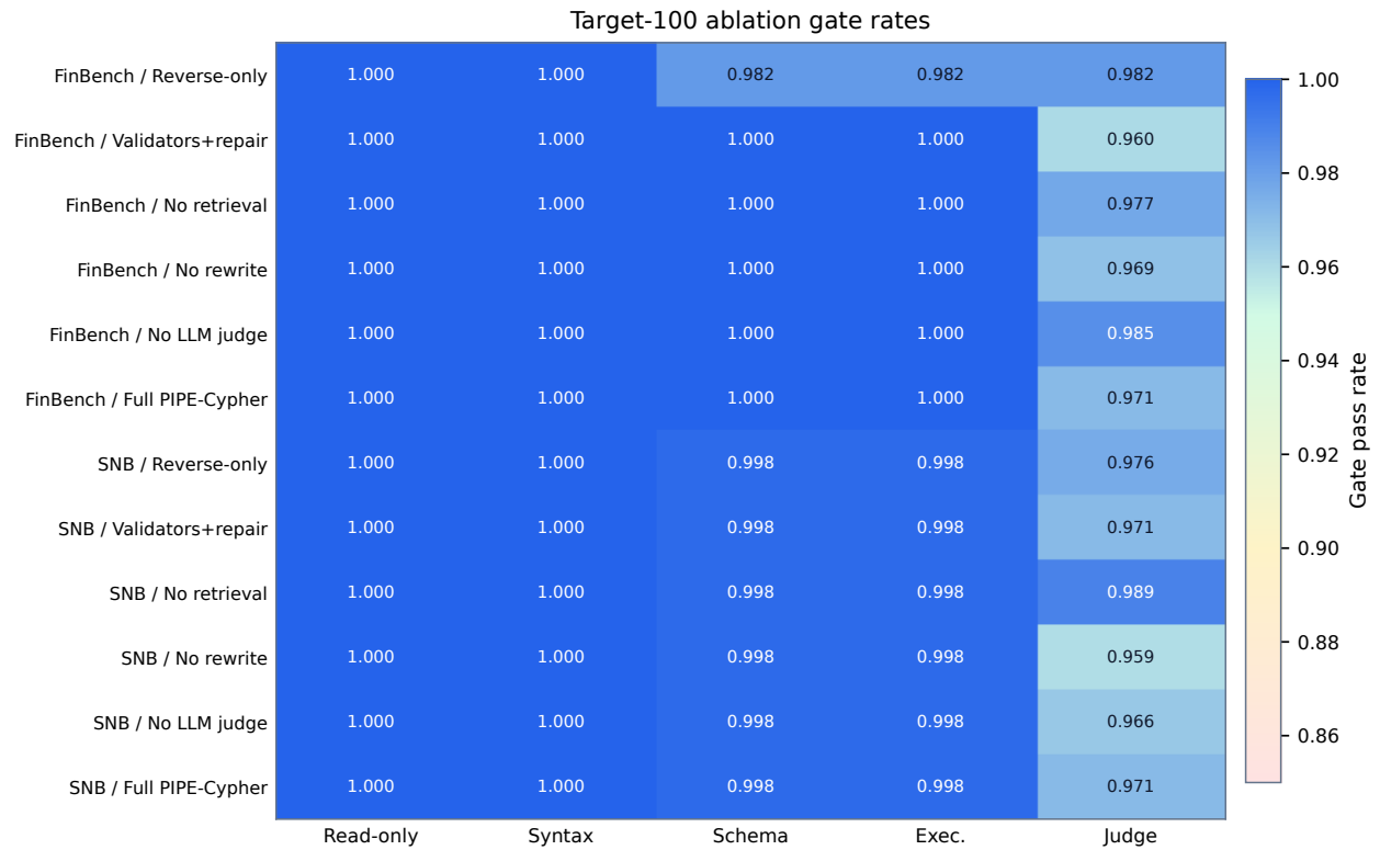
Figure 4: Gate-rate heatmap for the audited target-100 ablation suite. Deterministic read-only and syntax gates are saturated; execution and judge rates expose the remaining quality differences across graph and pipeline variants.
