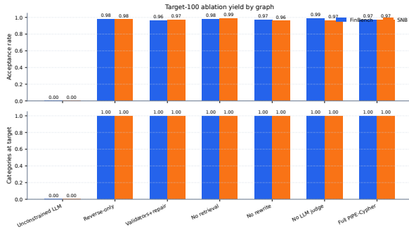
Figure 3: Audited target-100 ablation suite over FinBench and SNB. Every non-unconstrained graph/setting cell reaches all eight category targets with 800 accepted examples per cell.
