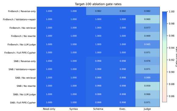
Figure 4: Gate-rate heatmap for the audited target-100 ablation suite. Deterministic read-only and syntax gates are saturated; execution and judge rates expose the remaining quality differences across graph and pipeline variants.
