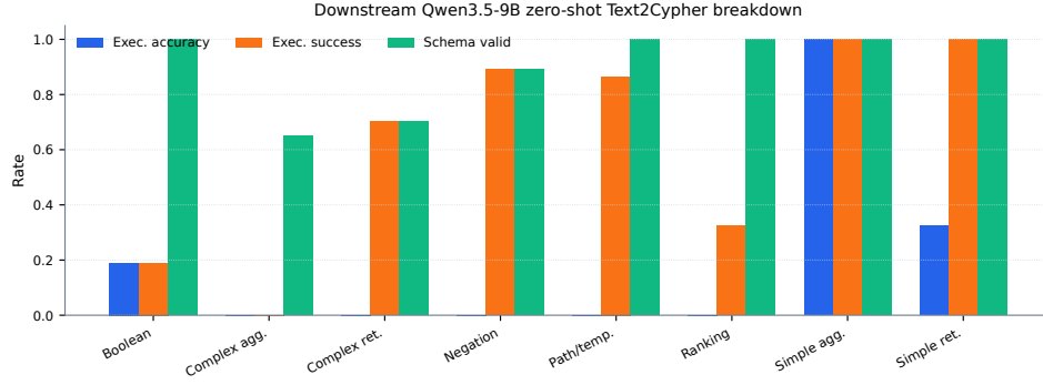
Figure 2: Downstream zero-shot Qwen3.5-9B Text2Cypher evaluation by workload category on the full test split. The benchmark separates parse/schema/execution success from exact execution accuracy, exposing operational categories where executable Cypher is still semantically wrong.
