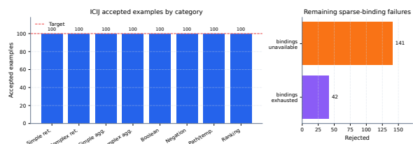
Figure 6: ICIJ Offshore Leaks onboarding audit. Schema-derived sparse-category templates recover balanced target-100 coverage on a public finance/compliance graph beyond the two LDDB workloads.
