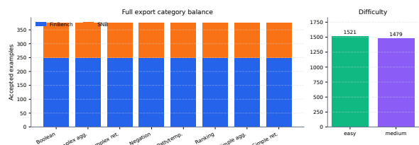
Figure 8: Full 3,000-example export distribution. The benchmark preserves the planned 2:1 FinBench/SNB graph mix while balancing all eight Cypher workload categories and maintaining a near-even easy/medium difficulty split.
