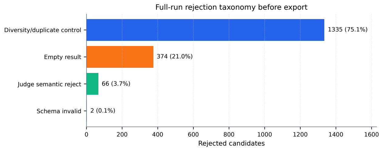
Figure 8: Full-run rejection taxonomy before benchmark export. Most rejected candidates come from duplicate/diversity control during category recovery and from empty execution results; schema-invalid Cypher is rare after deterministic governance.
