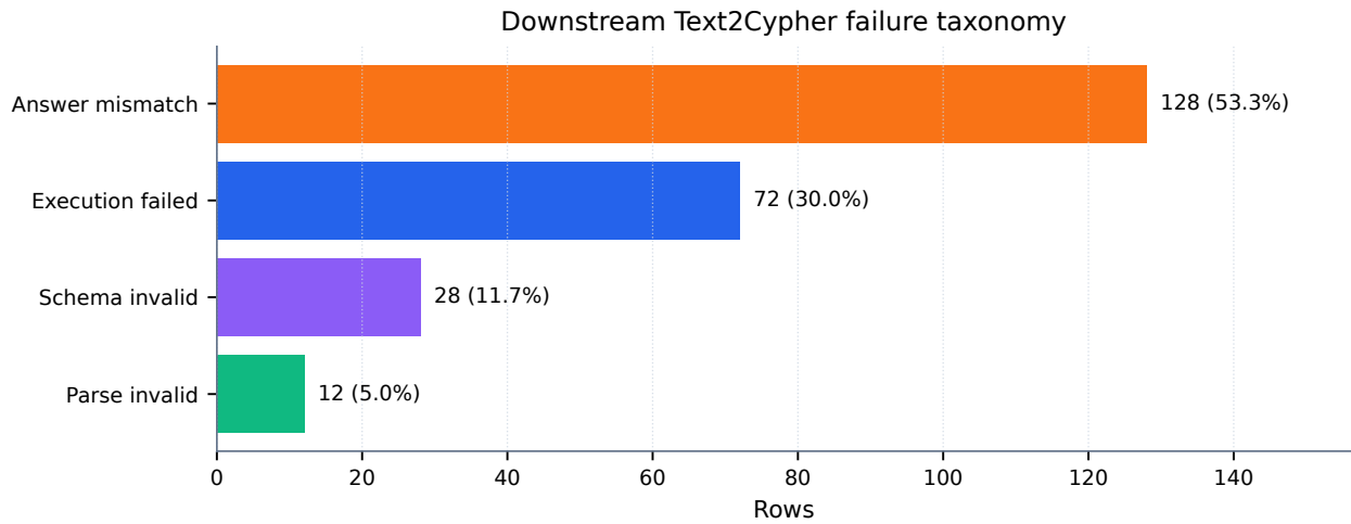
Figure 7: Downstream Text2Cypher failure taxonomy for the local Qwen3.5-9B baseline on the full test split. Exact matches are excluded so the chart exposes whether misses come from invalid Cypher, failed execution, or semantically wrong executable queries.
