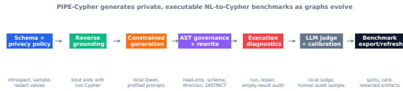
Figure 1: PIPE-Cypher benchmark generation pipeline. The key industry additions beyond static Text2Cypher dataset construction are privacy/value policies, reverse grounding, Cypher governance, execution diagnostics, local judge calibration, and benchmark export/refresh.
