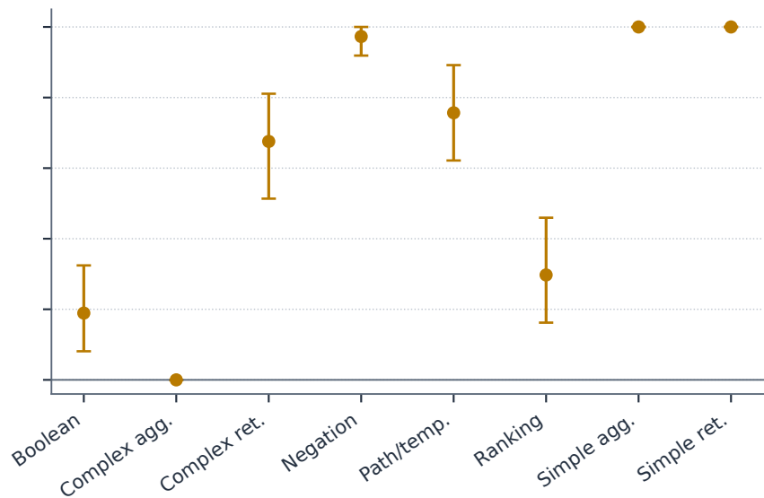
Execution success
