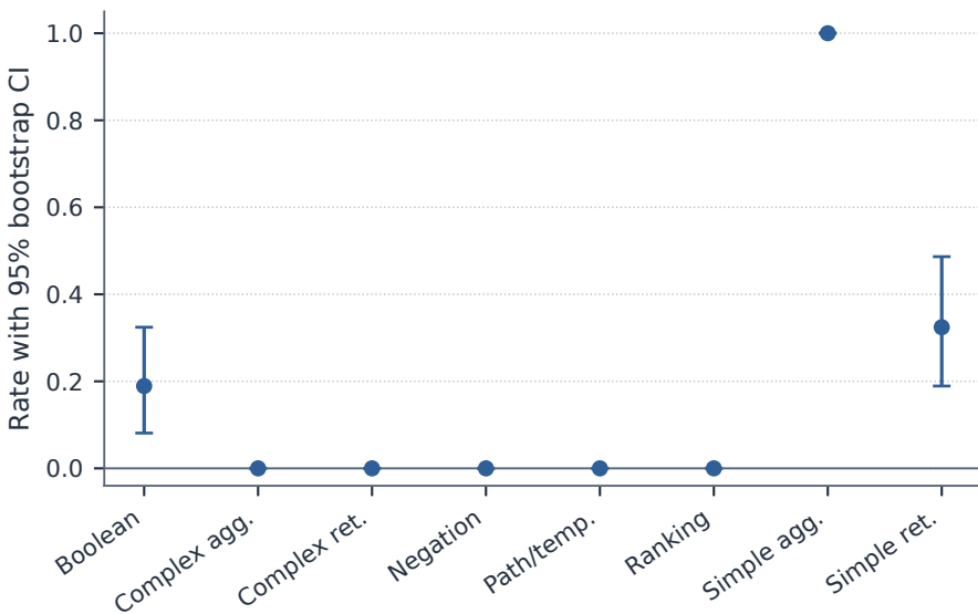
Execution accuracy
