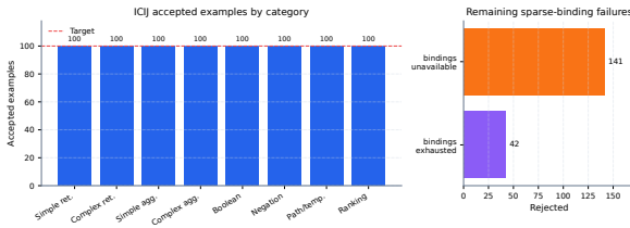
Figure 5: ICIJ Offshore Leaks onboarding audit. Schema-derived sparse-category templates recover balanced target-100 coverage on a public finance/compliance graph beyond the two LDBC workloads.
