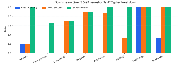
Figure 5: Downstream zero-shot Qwen3.5-9B Text2Cypher evaluation by workload category on the full test split. The breakdown separates final execution accuracy from parse/schema/execution success signals, making difficult operational categories visible.
