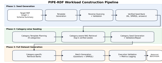
Figure 1: PIPE-RDF workload-construction pipeline: Phase 1 uses reverse query generation to build verified seeds; Phase 2 constructs category-specific seed banks; Phase 3 generates the balanced benchmark with execution-driven validation/repair.
