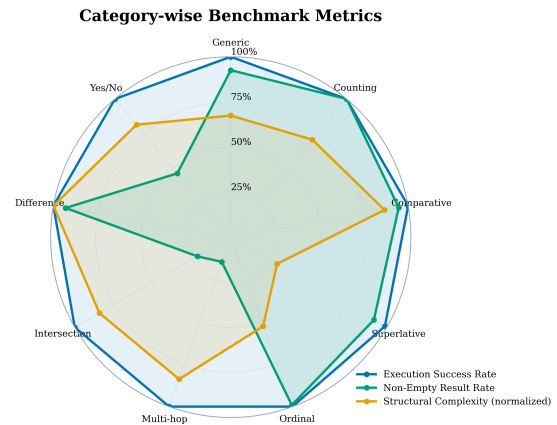
Figure 2: Category-wise metrics: execution success (100%), non-empty rate, and normalized structural complexity.
