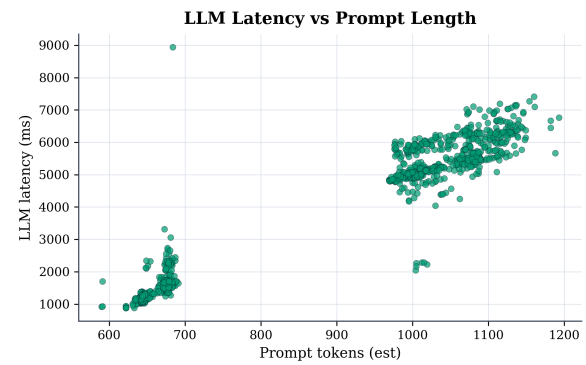
Figure 9: Prompt length distribution and latency vs. prompt length.
