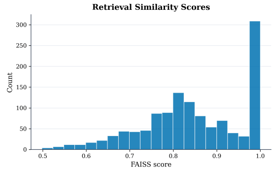
Figure 7: Distribution of retrieval similarity scores.
