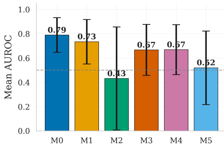
(b) Mean AUROC
