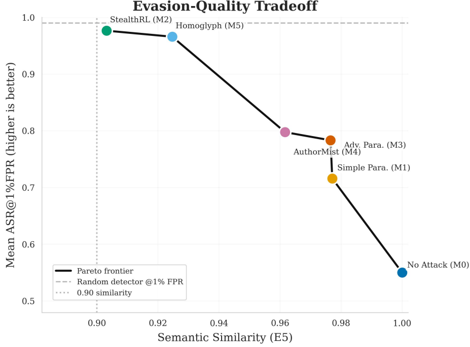
Figure 6: Evasion-quality tradeoff at the 1% FPR operating point. Each point represents a method, plotted by E5 semantic similarity (x-axis) against mean ASR@1%FPR (y-axis). Top-right is ideal (high similarity, high attack success). The dashed lines mark the 0.90 similarity floor and the random-detector ASR baseline at 1% FPR, and the solid line shows the Pareto frontier.
