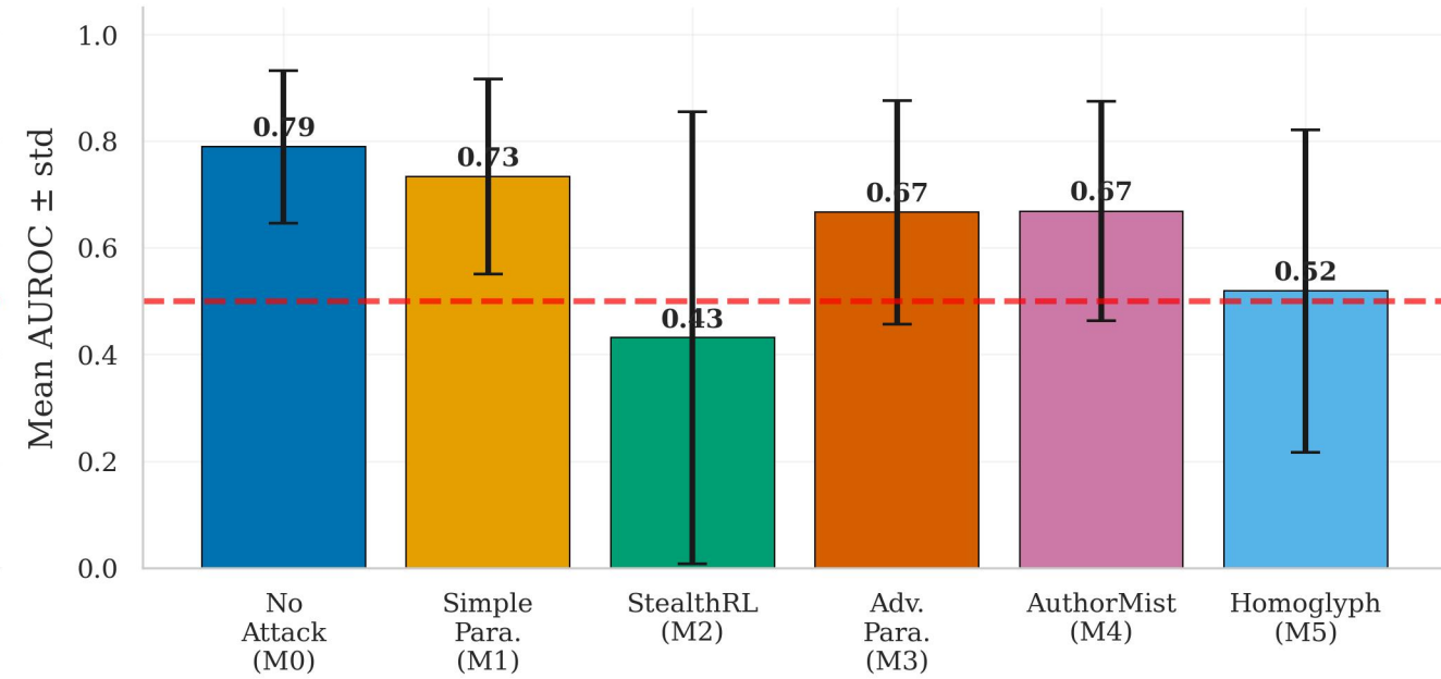
(b) Mean AUROC Across Detectors
