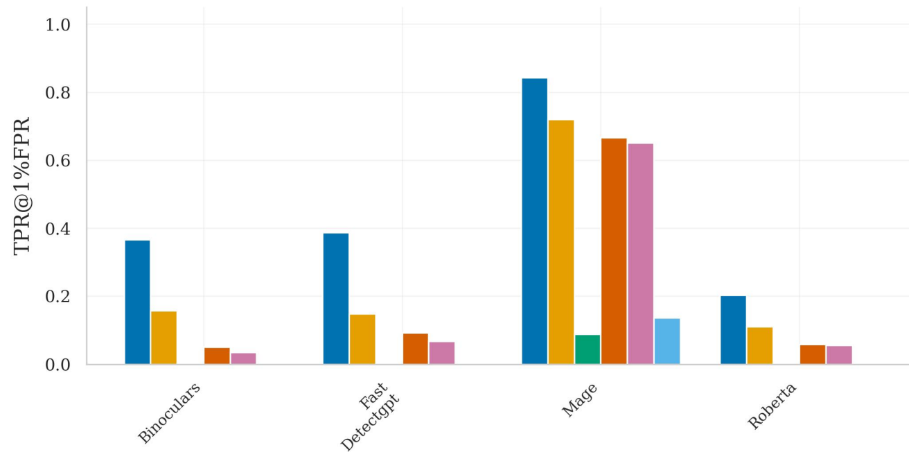
(c) True Positive Rate at 1% FPR
