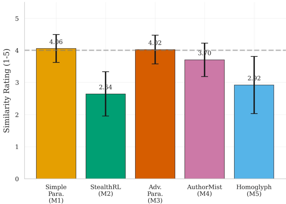
(b) Semantic Similarity
