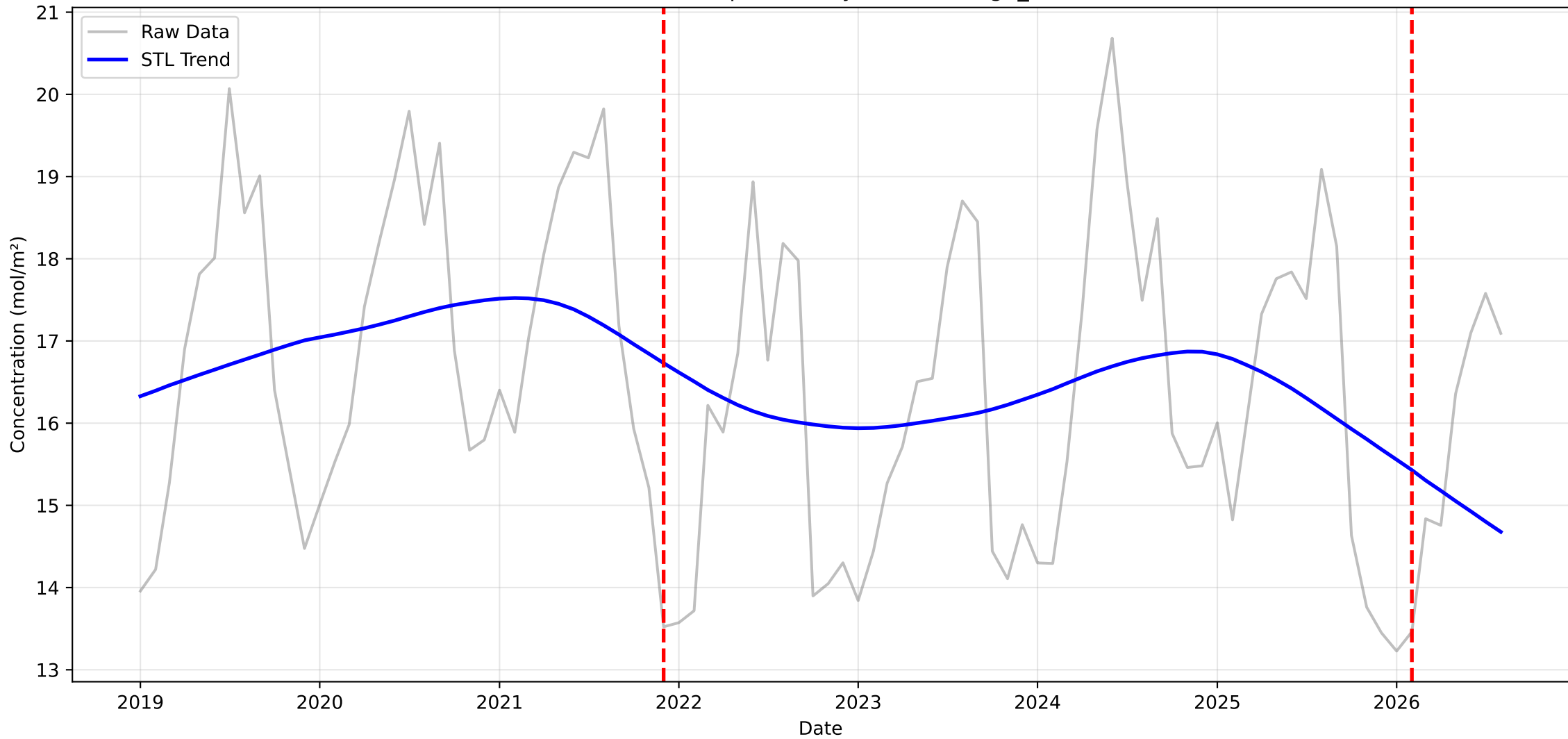
Structural Breakpoint Analysis: CO in High_Himal
