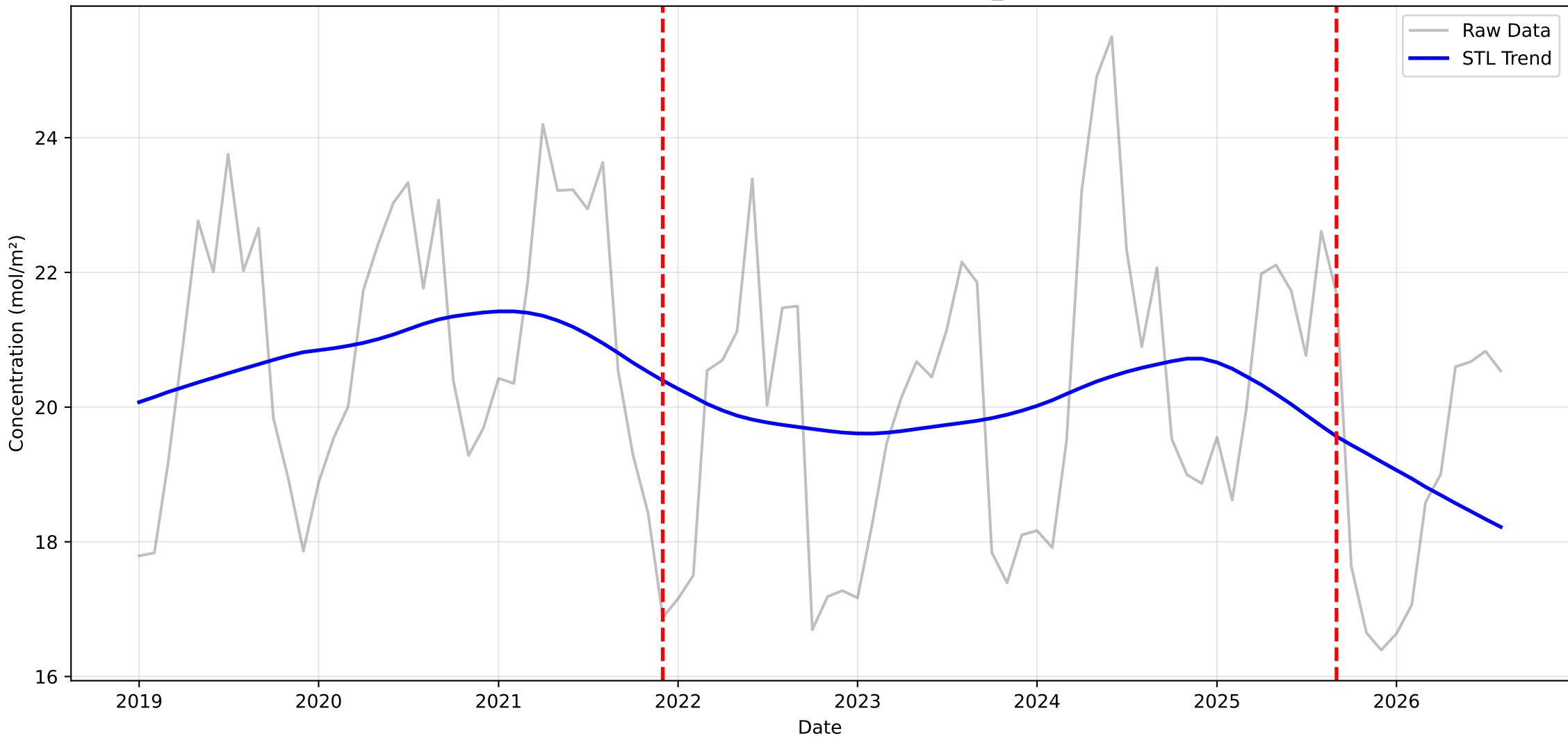
Structural Breakpoint Analysis: CO in High_Mountains
