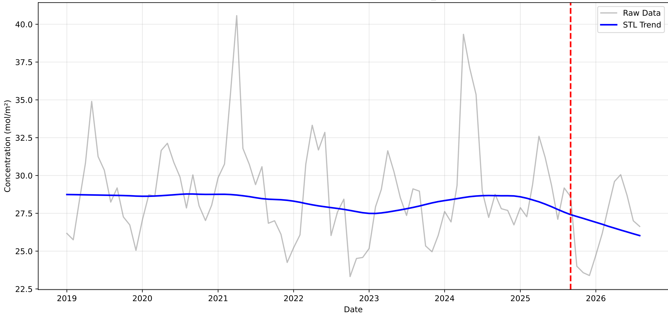
Structural Breakpoint Analysis: CO in Middle_Mountains
