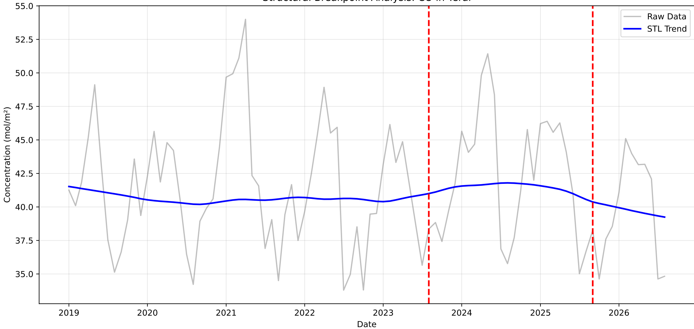
Structural Breakpoint Analysis: CO in Terai
