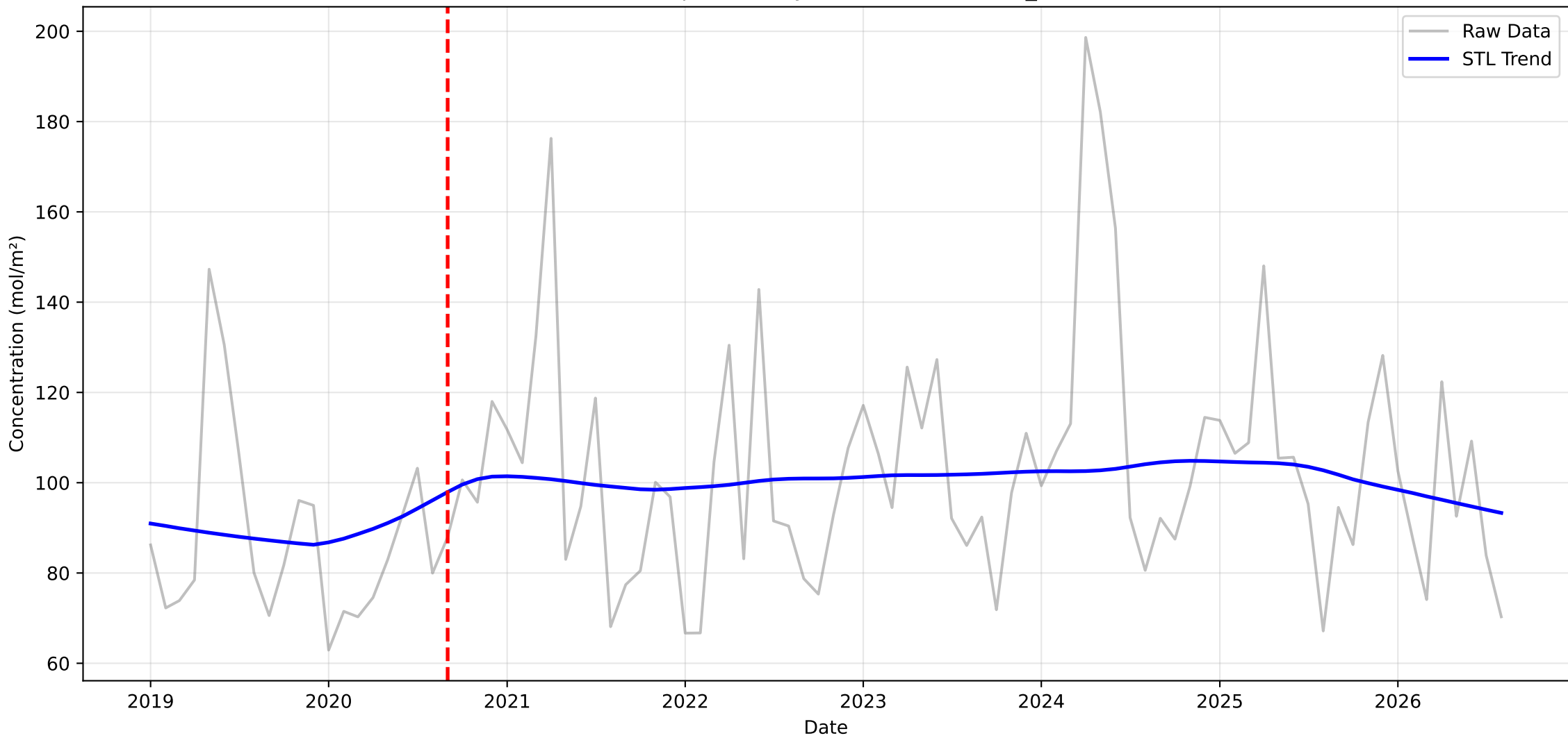
Structural Breakpoint Analysis: HCHO in Middle_Mountains
