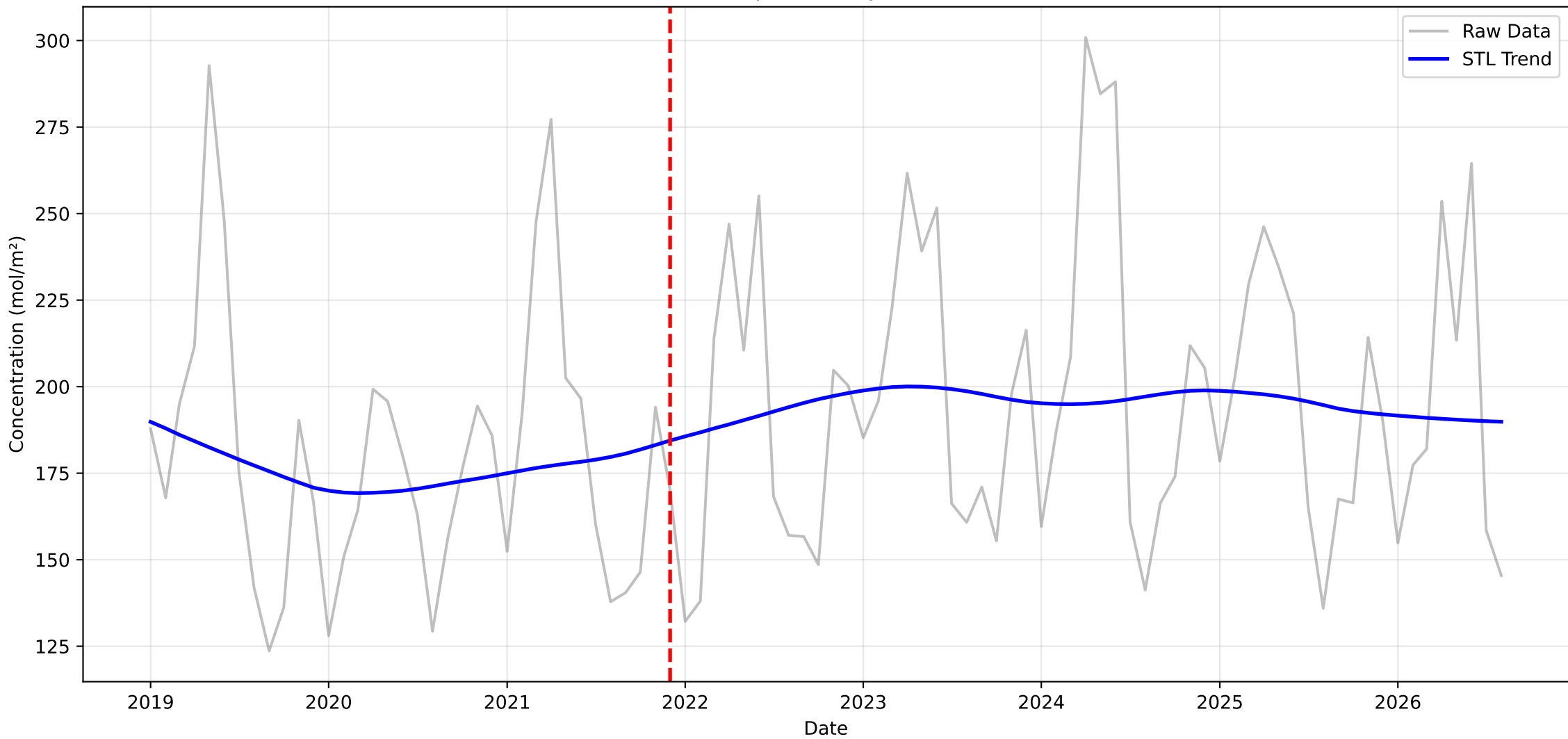
Structural Breakpoint Analysis: HCHO in Terai
