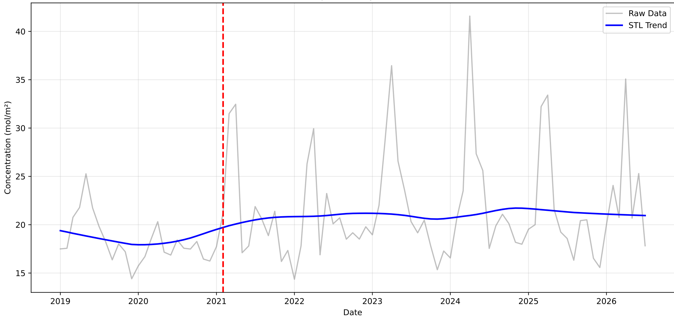
Structural Breakpoint Analysis: NO2 in Siwalik
