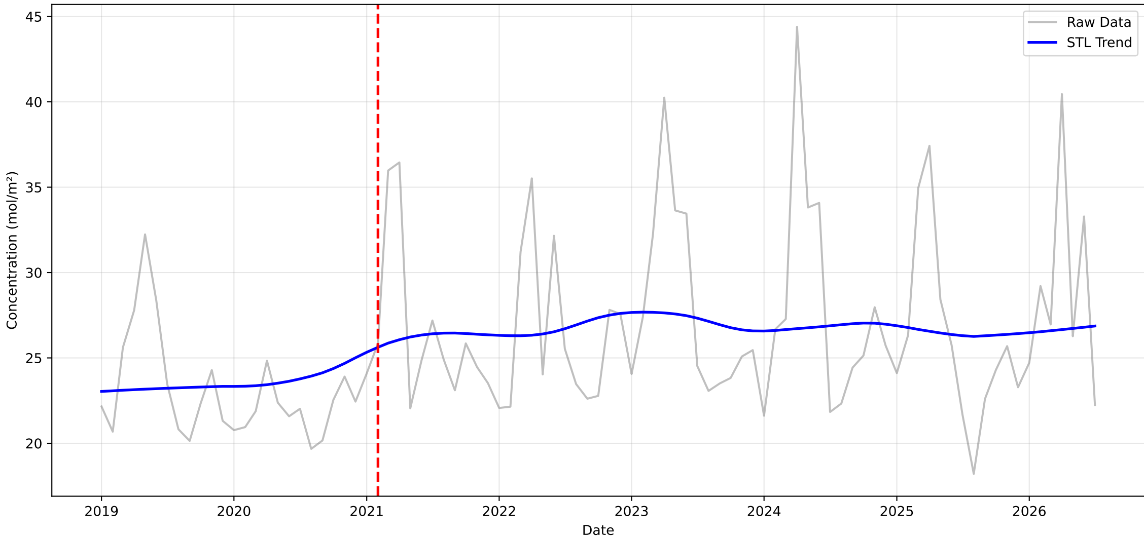
Structural Breakpoint Analysis: NO2 in Terai
