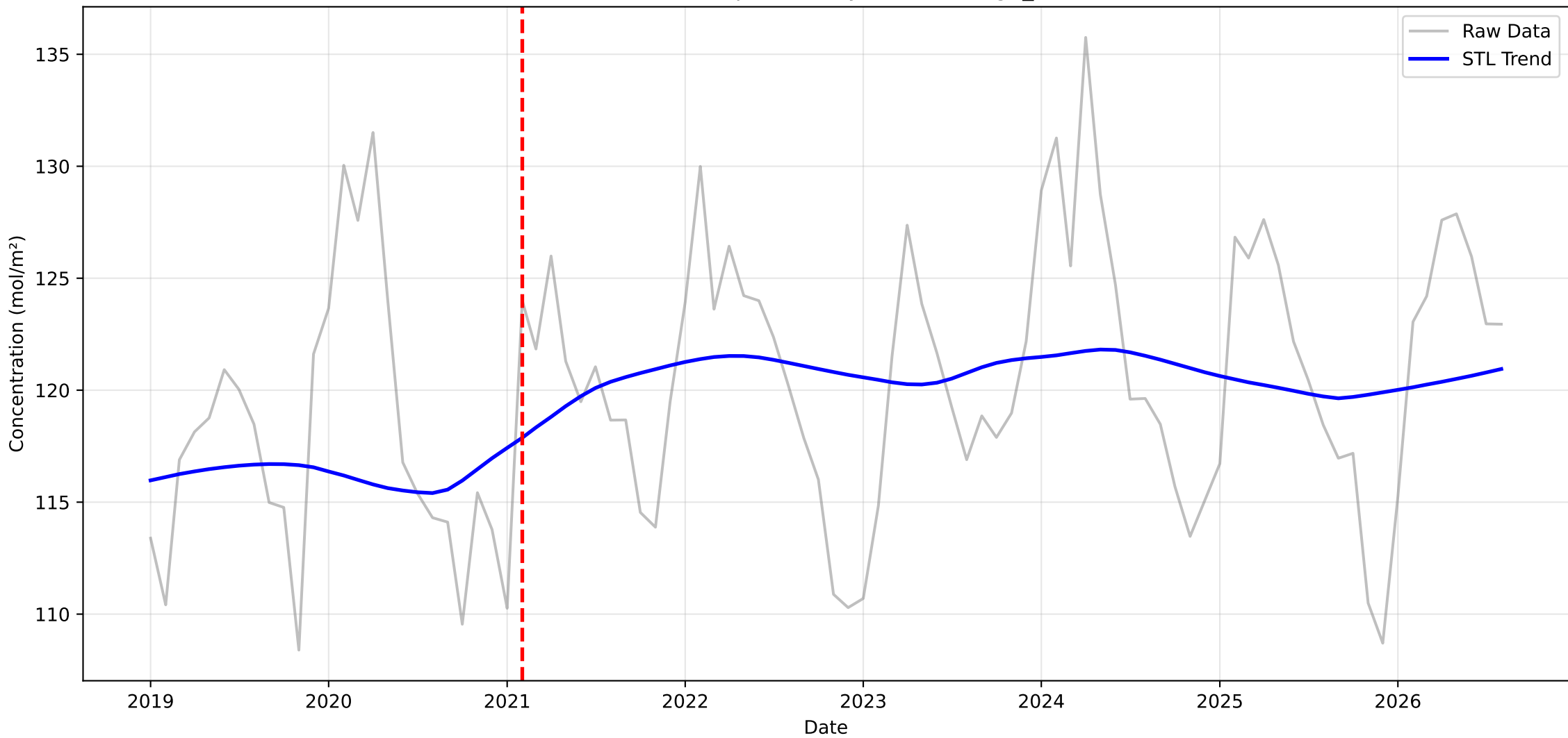
Structural Breakpoint Analysis: O3 in High_Himal
