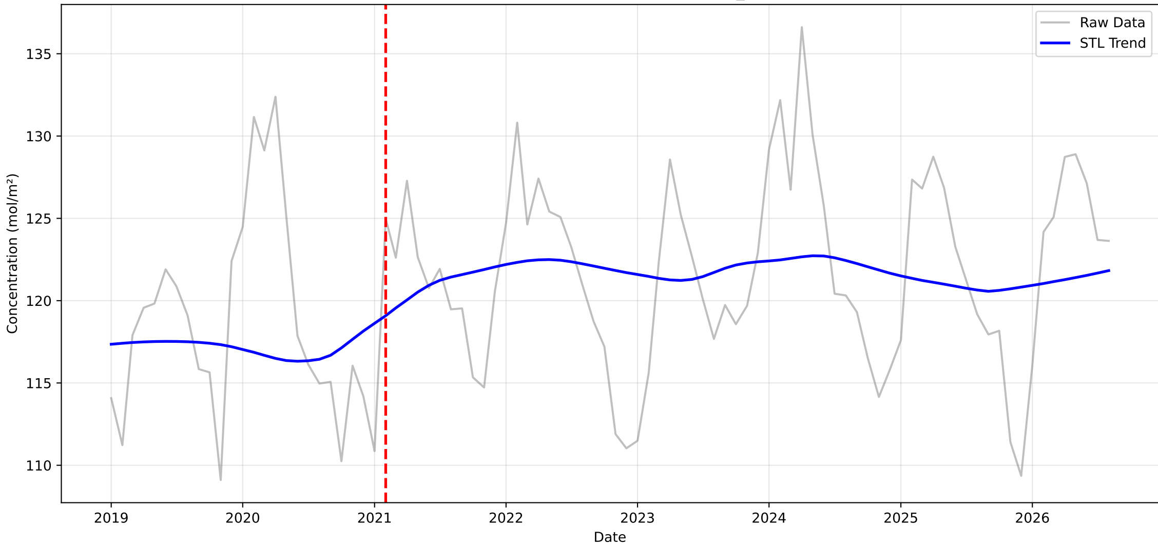
Structural Breakpoint Analysis: O3 in High_Mountains
