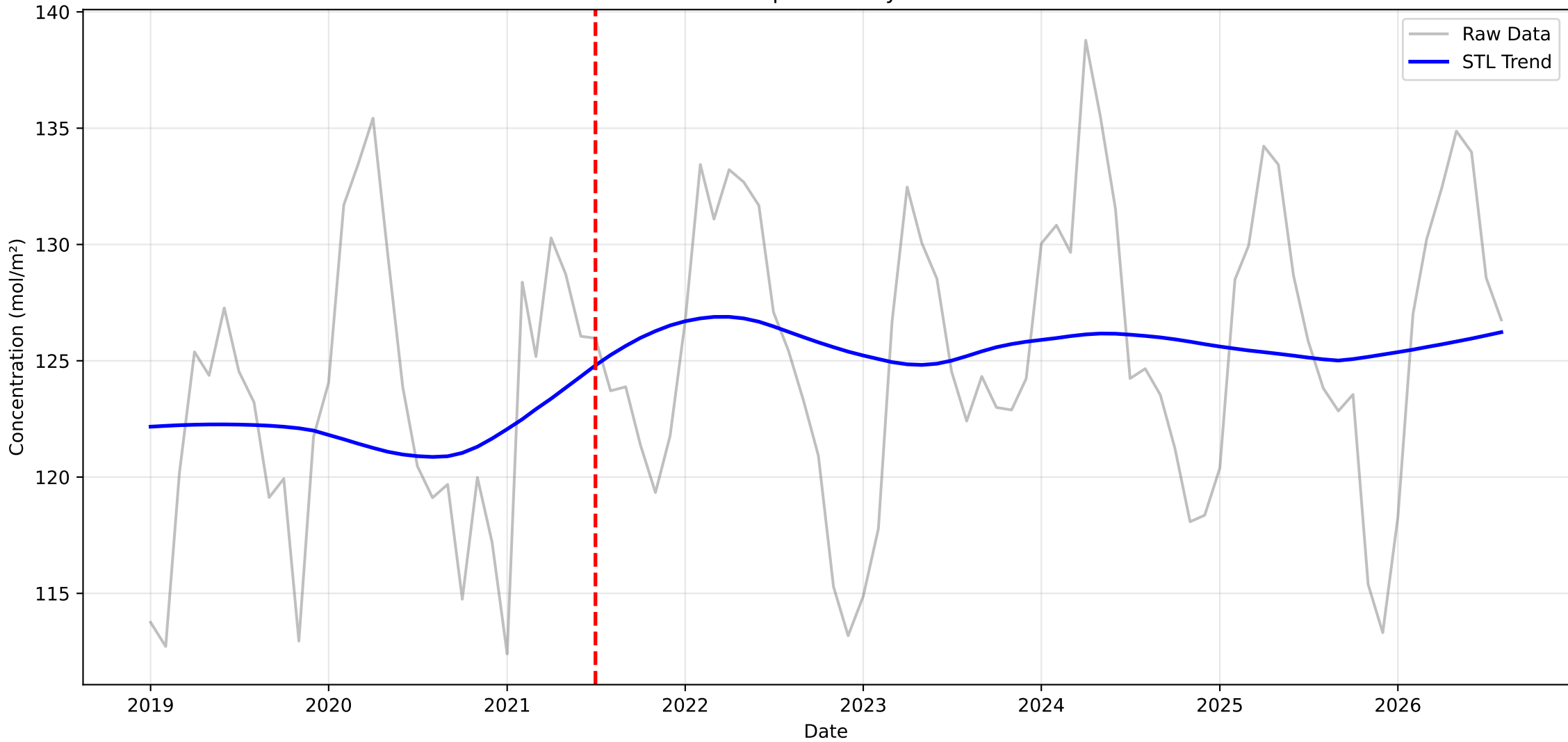
Structural Breakpoint Analysis: O3 in Terai
