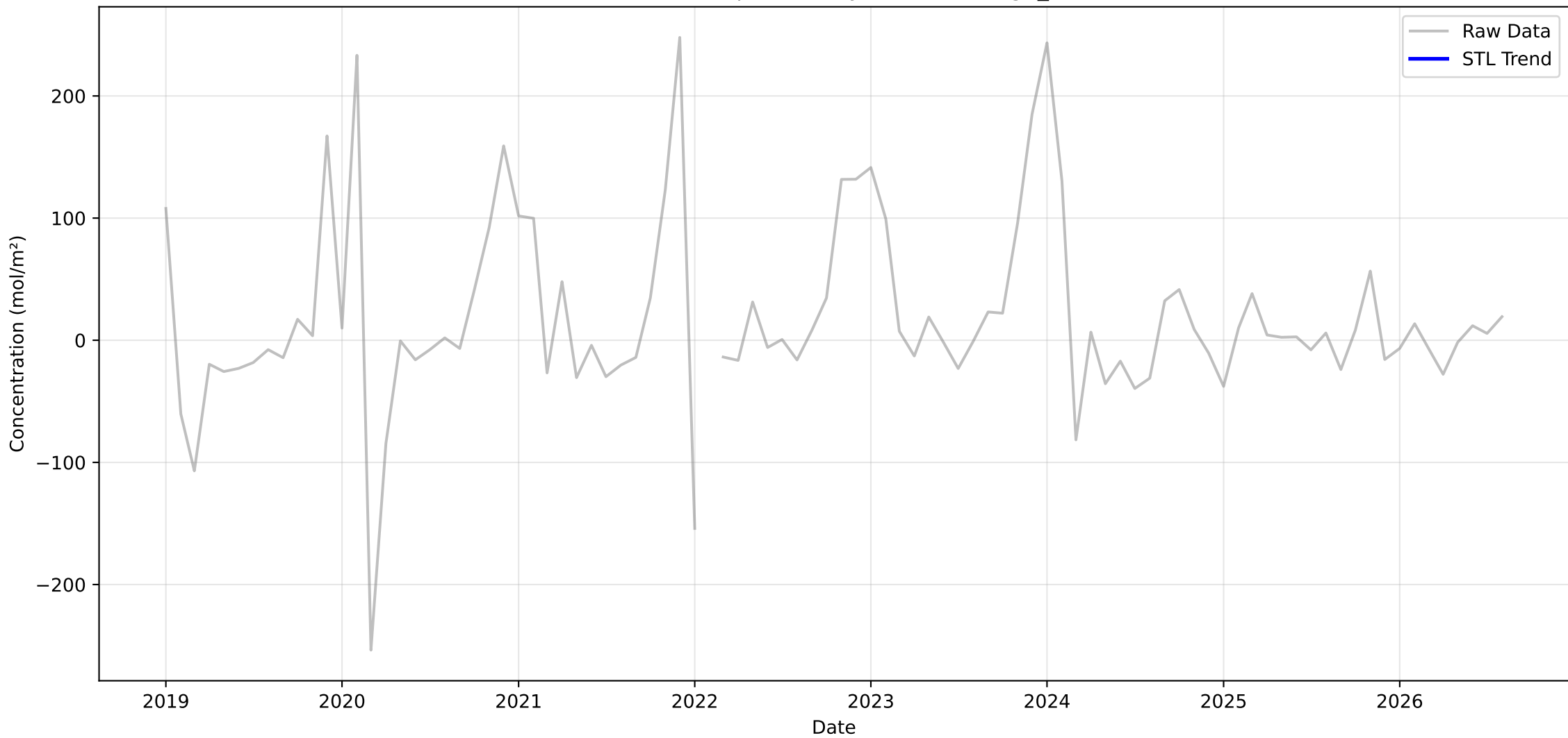
Structural Breakpoint Analysis: SO2 in High_Himal
