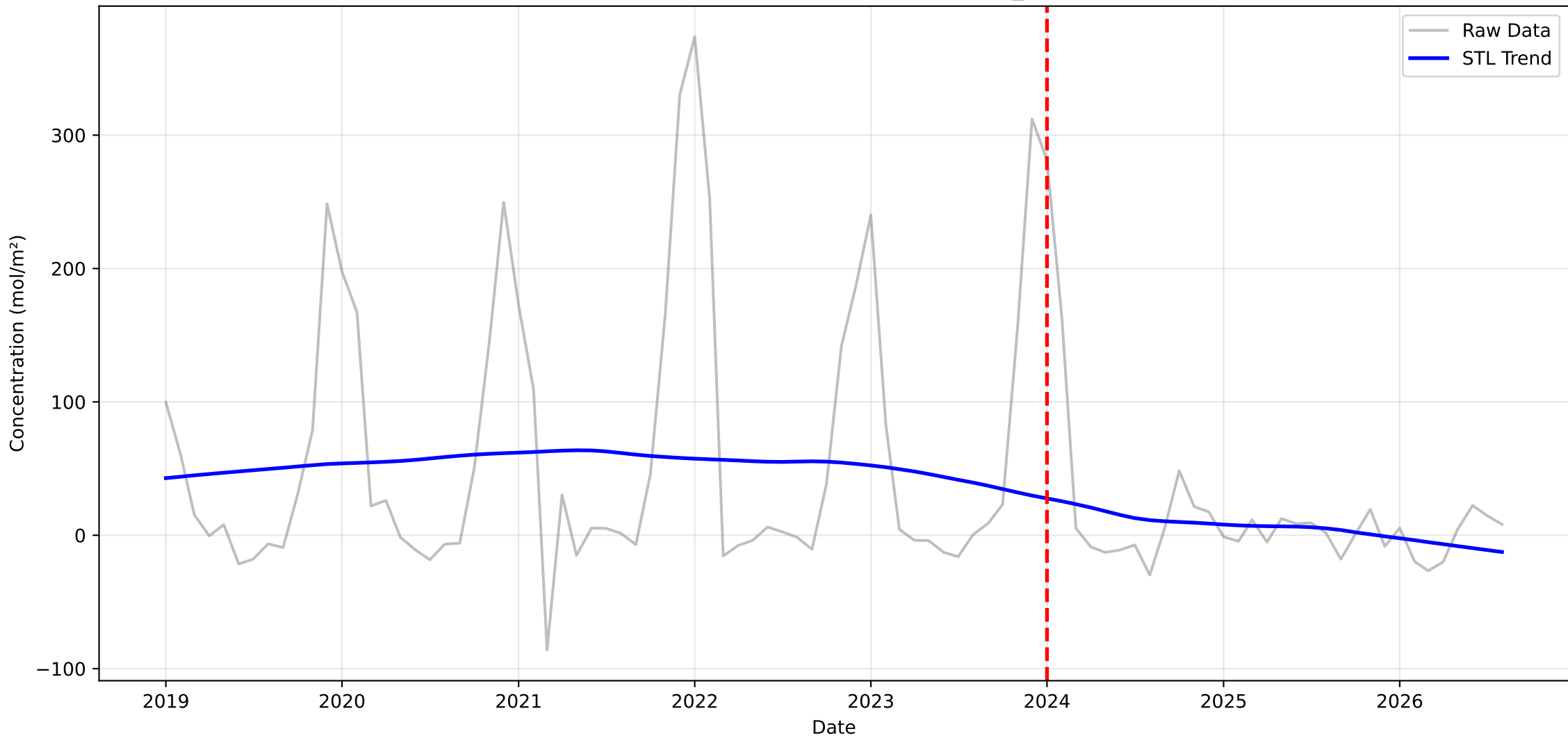
Structural Breakpoint Analysis: SO2 in High_Mountains
