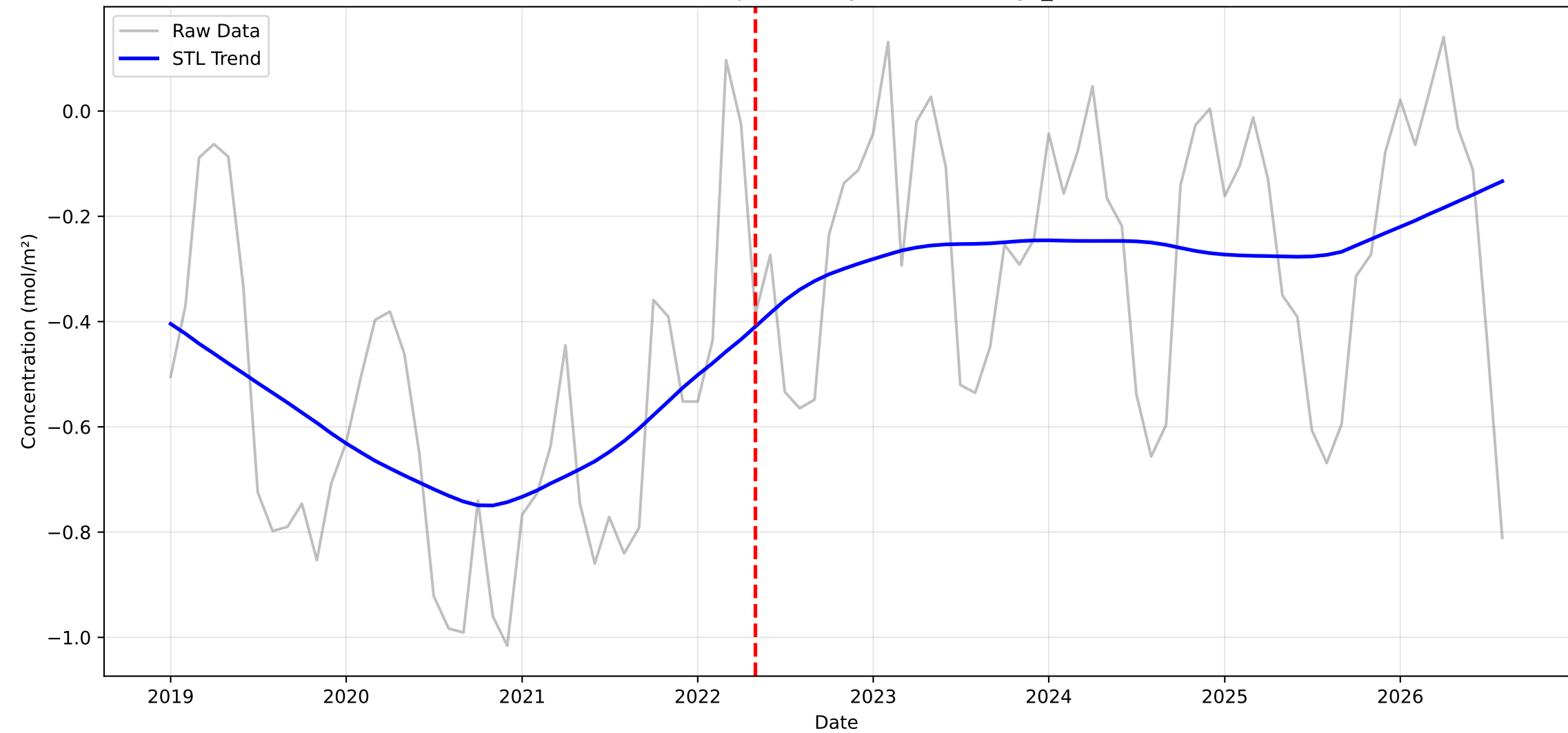
Structural Breakpoint Analysis: UVAI in High_Himal
