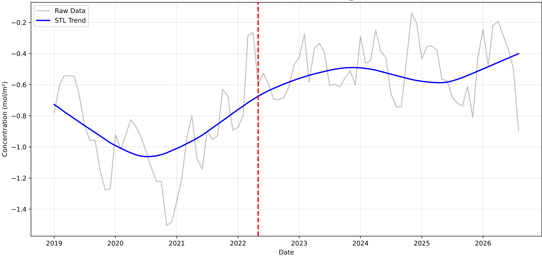
Structural Breakpoint Analysis: UVAI in High_Mountains
